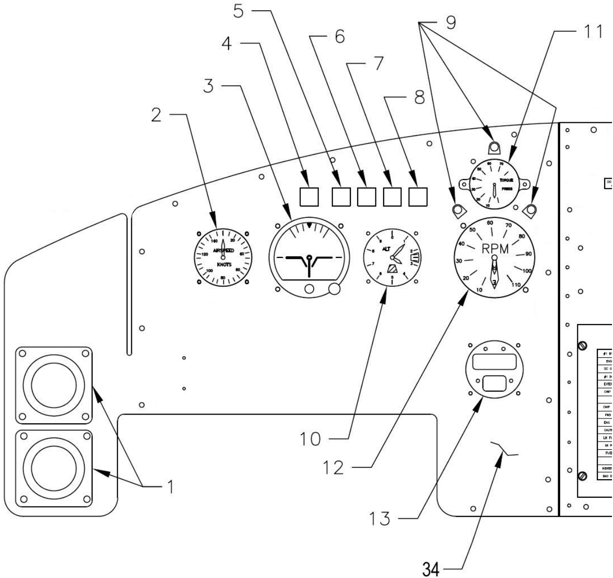
Figure 95-1 Instrument Panel Assembly (Sheet 1 of 3) (S/N's 30687, 30931, 30576, 30817 and 30599)
