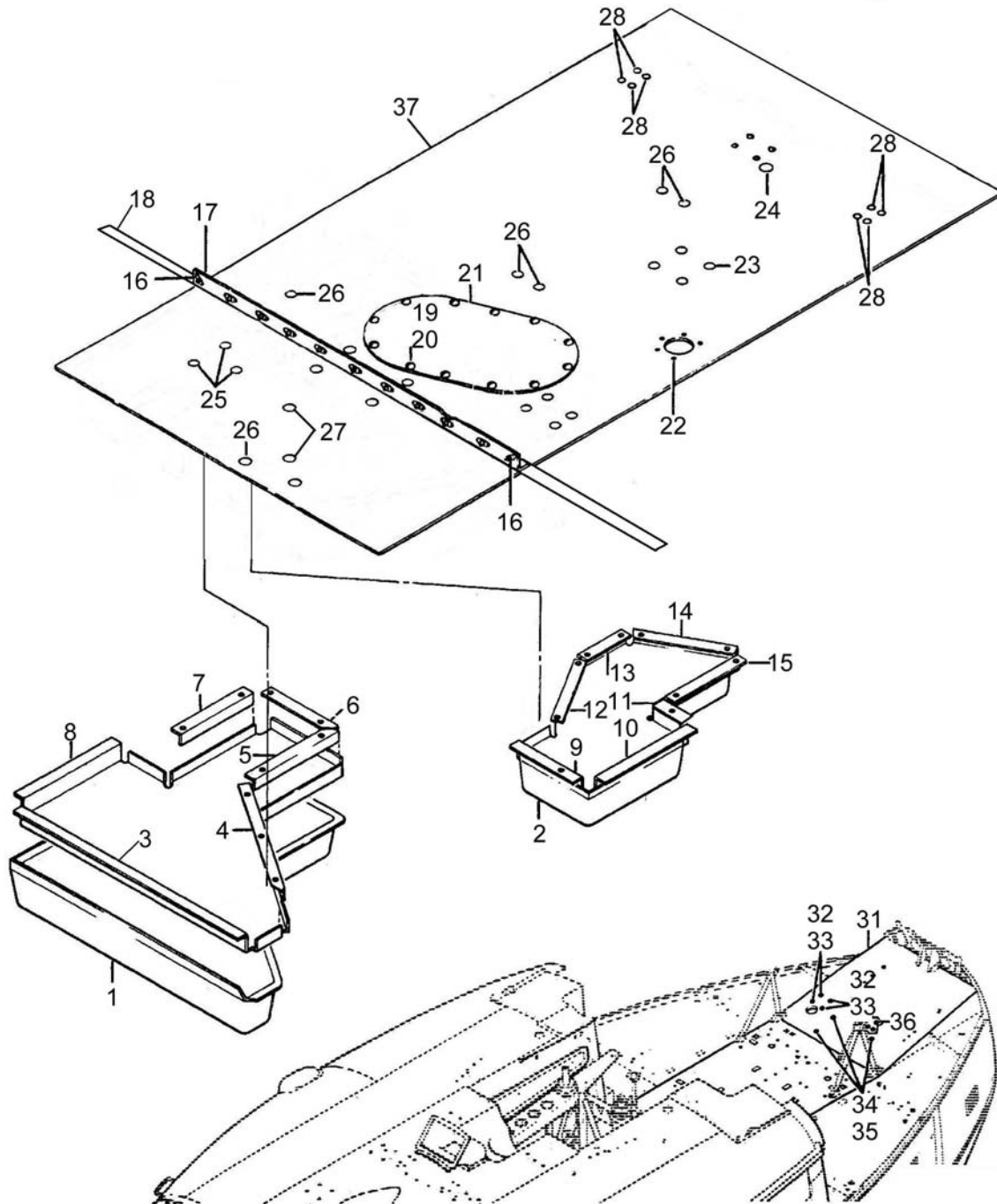
Figure 53-8 Engine Deck (Sheet 1 of 2)
