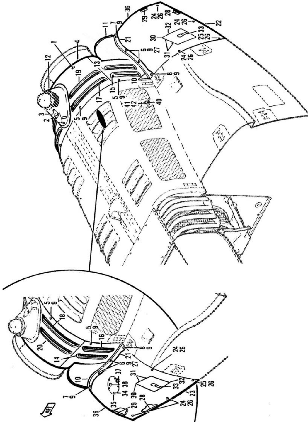
Figure 71-5 Cowl Installation
