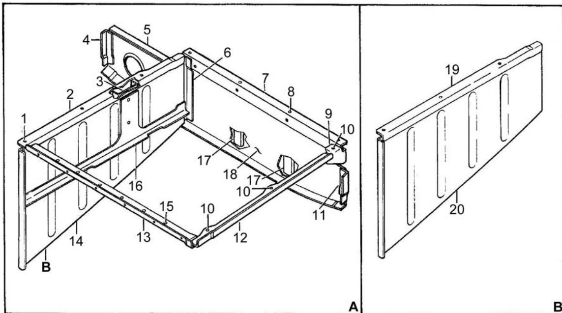
Figure 53-16 Oil Cooler Support
