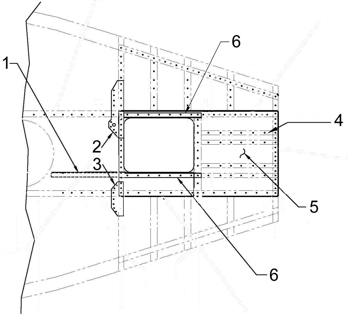
Figure 53-5 Belly Skin Installation (All aircraft except s/n 30687, 30931, 30576, 30817 and 30599)
