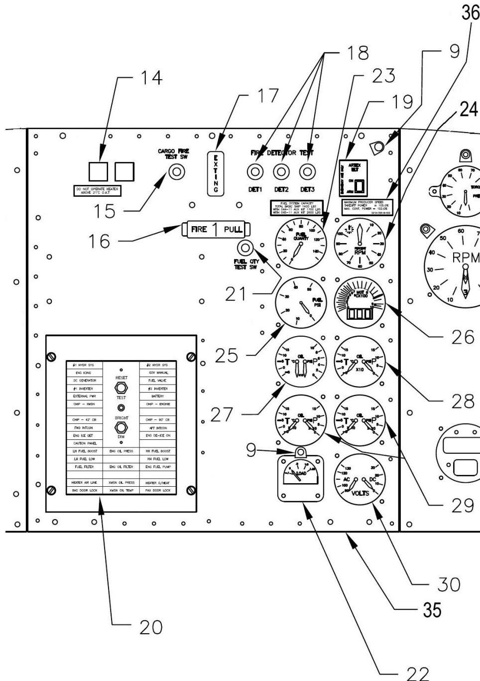
Figure 95-1 Instrument Panel Assembly (Sheet 2 of 3) (S/N's 30687, 30931, 30576, 30817 and 30599)
