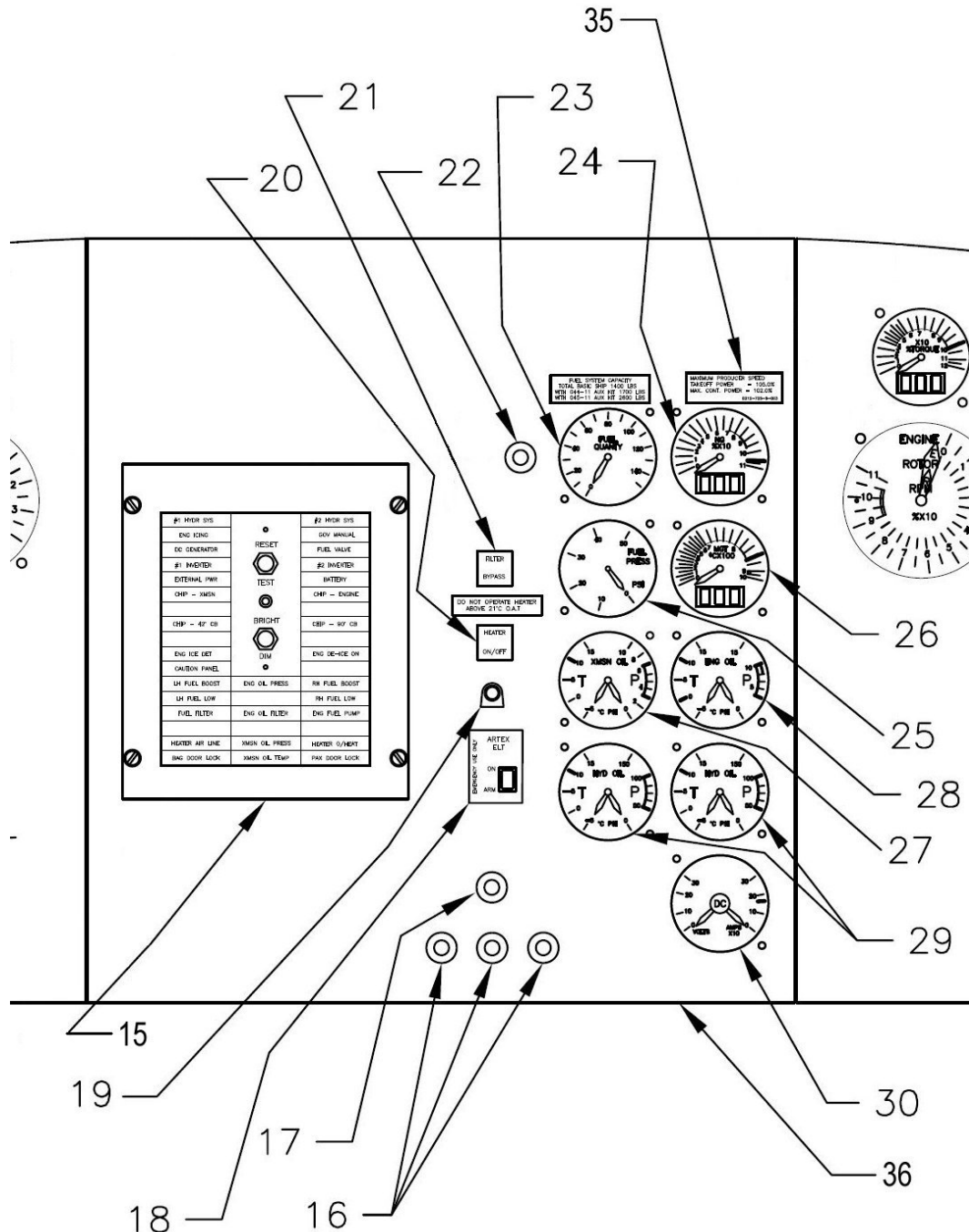
Figure 95-2 Instrument Panel Assembly (Sheet 2 of 3) (All S/N's except 30687, 30931, 30576, 30817, and 30599)
