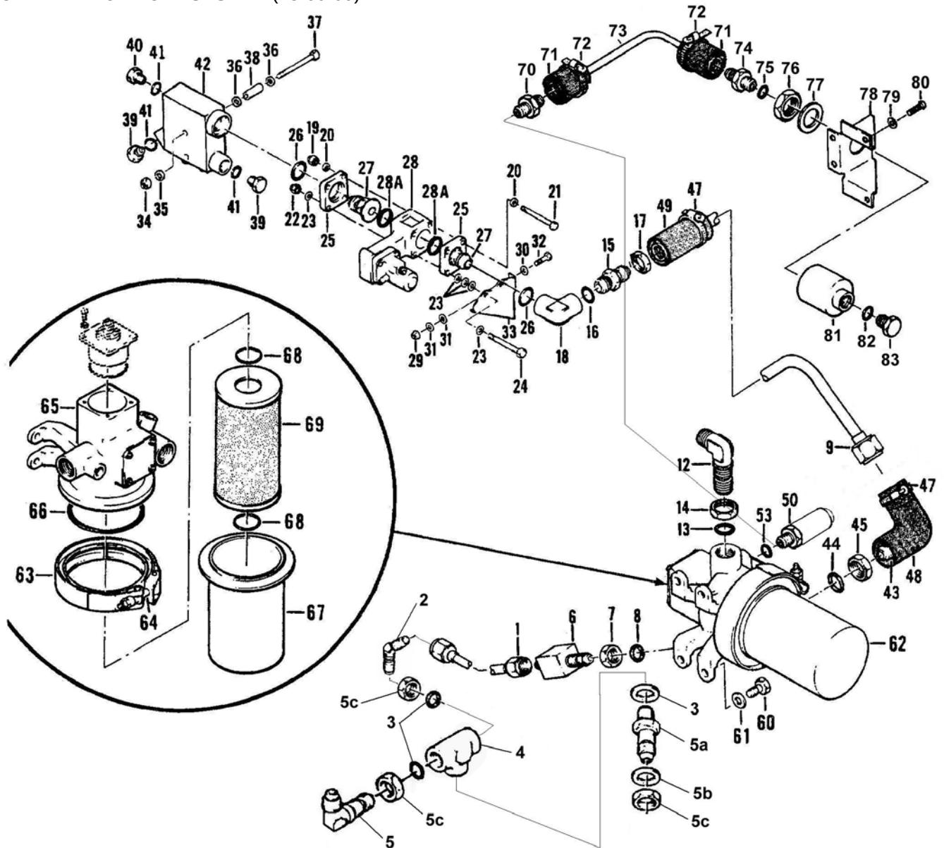
Figure 28-3 Fuel Filter and Firewall Shut Off
