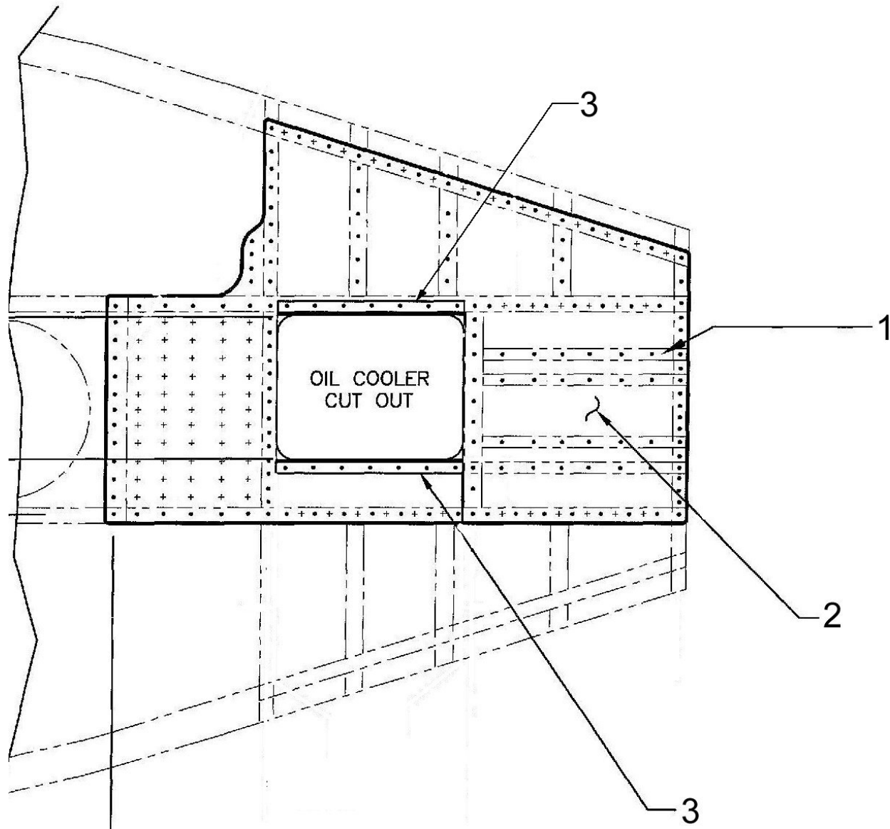
Figure 53-4 Belly Skin Installation (s/n 30599)
