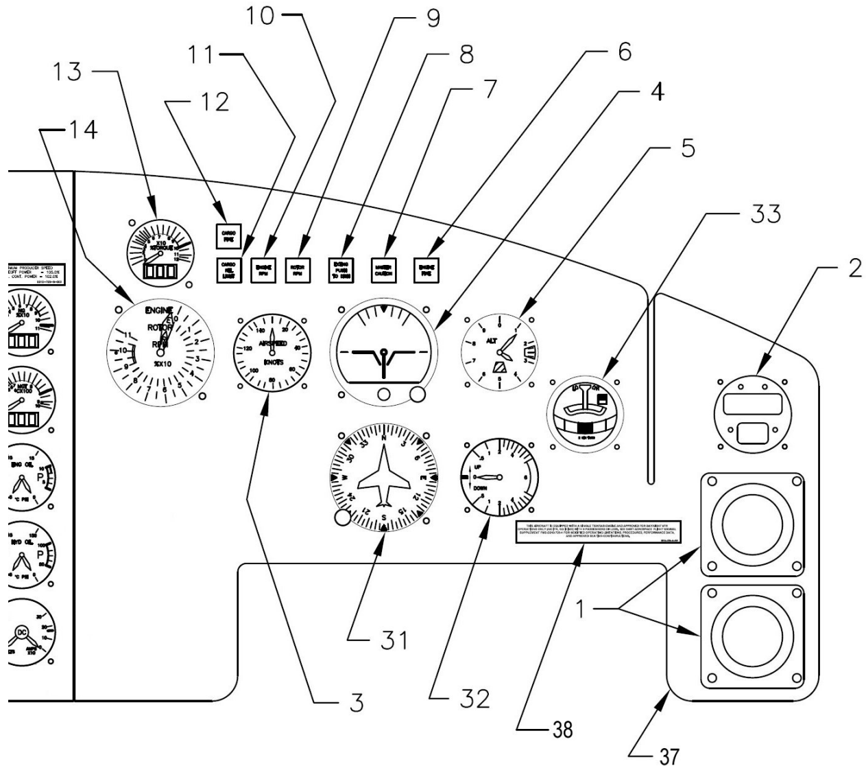
Figure 95-2 Instrument Panel Assembly (Sheet 3 of 3) (All S/N's except 30687, 30931, 30576, 30817, and 30599)
