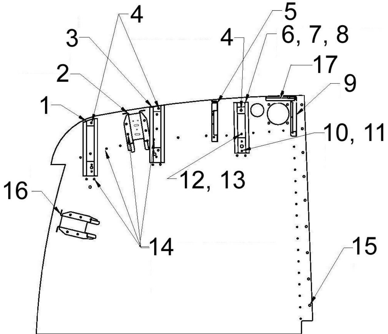
Figure 53-13 Bulkhead Installation
