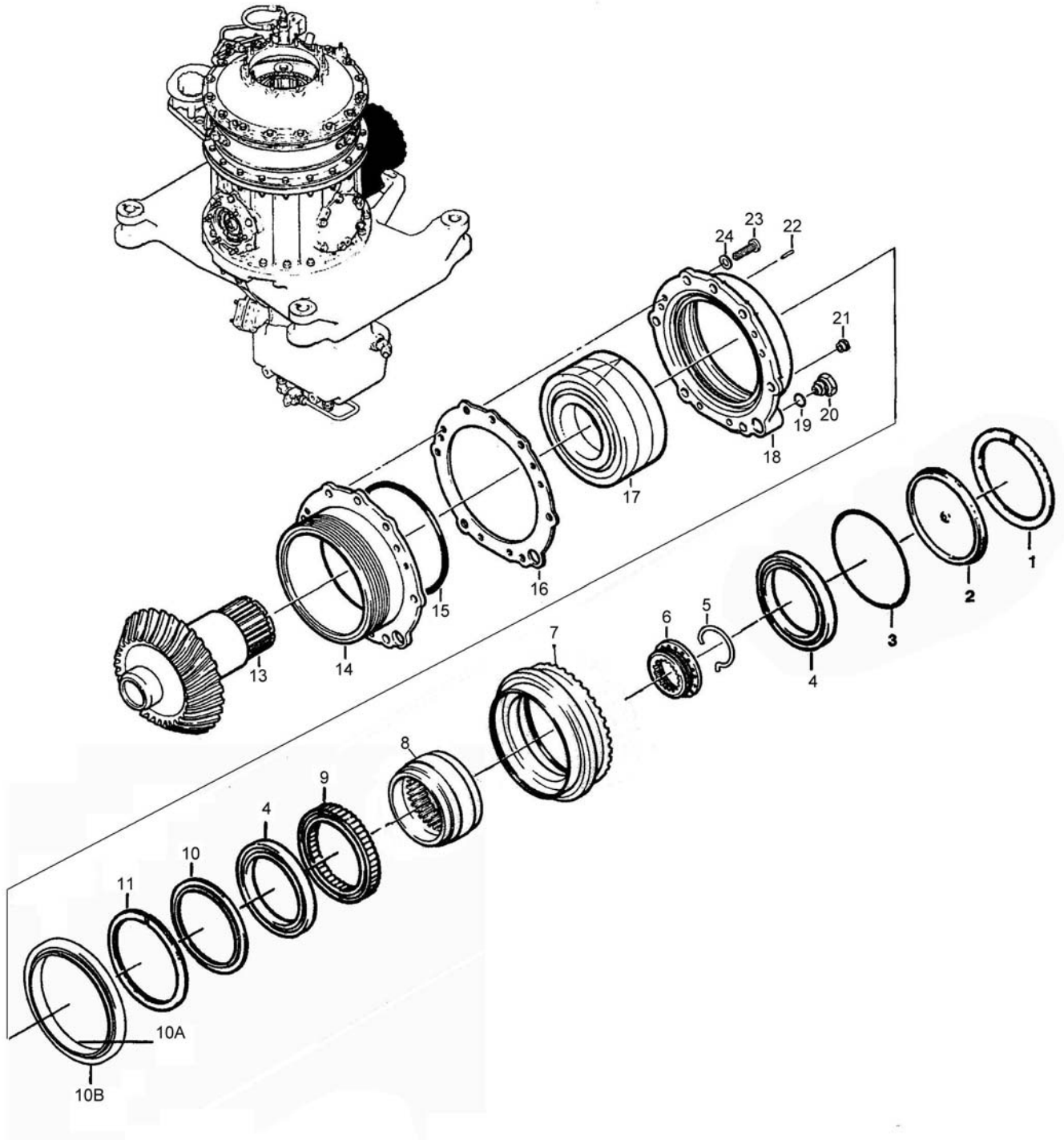
Figure 63-4 205-040-263-101 Quill Assembly
