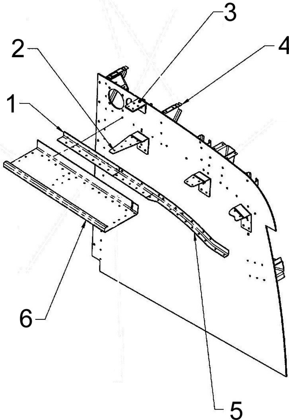
Figure 53-14 Bulkhead Installation
