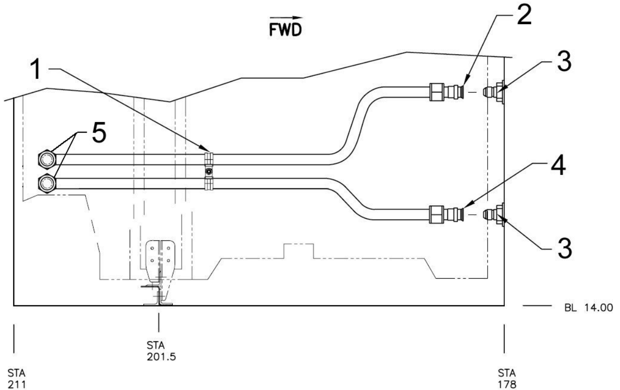
Figure 53-23 Vent Tube Installation (All S/N's Except 30687, 30931, 30576, 30817, 30599 and 30544)
