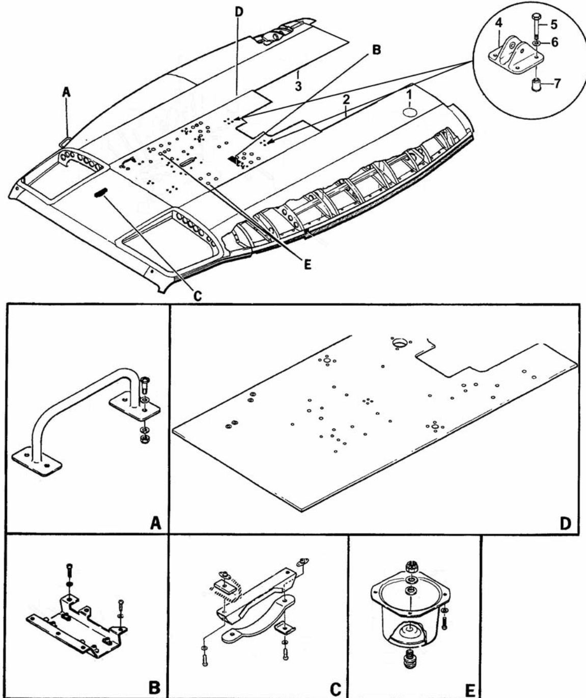
Figure 53-1 Roof Assembly
