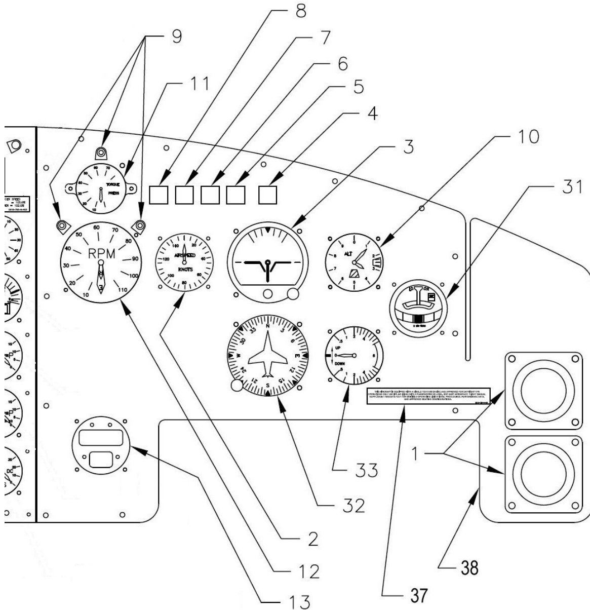
Figure 95-1 Instrument Panel Assembly (Sheet 3 of 3) (S/N's 30687, 30931, 30576, 30817 and 30599)
