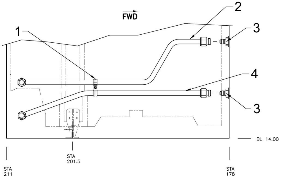
Figure 53-22 Vent Tube Installation (S/N 30687, 30931, 30576, 30817, 30599 and 30544)
