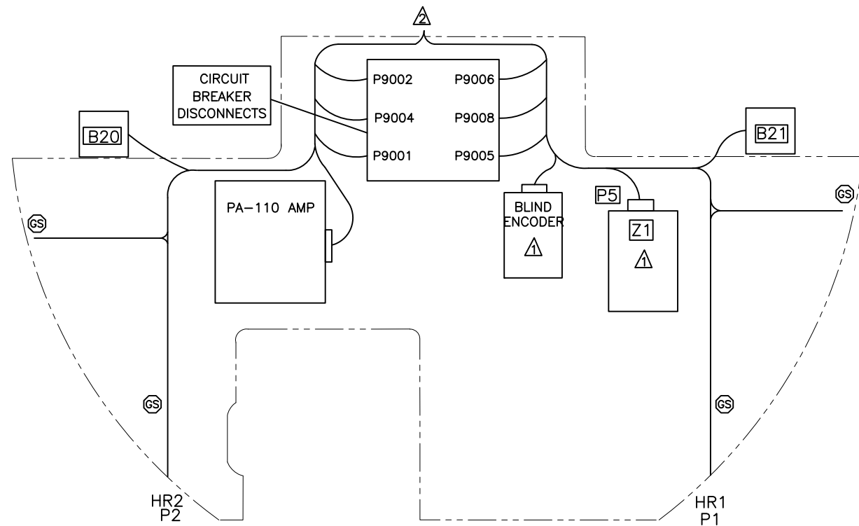
UPPER SHELF – TOP SIDE
