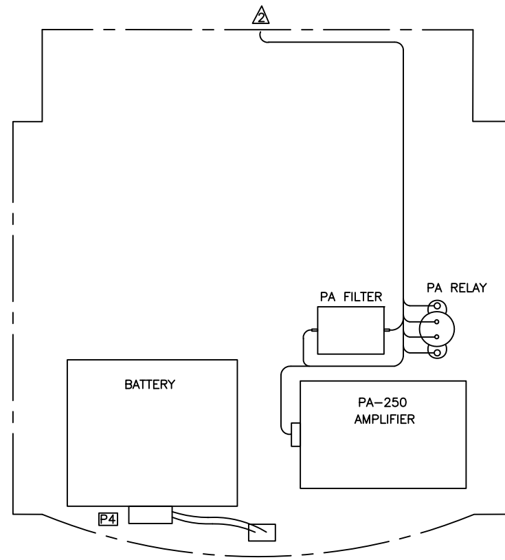
LOWER SHELF – BOTTOM SIDE (EFFECTIVE ON ALL S/N, EXCEPT 30687, 30817 & 30599)
