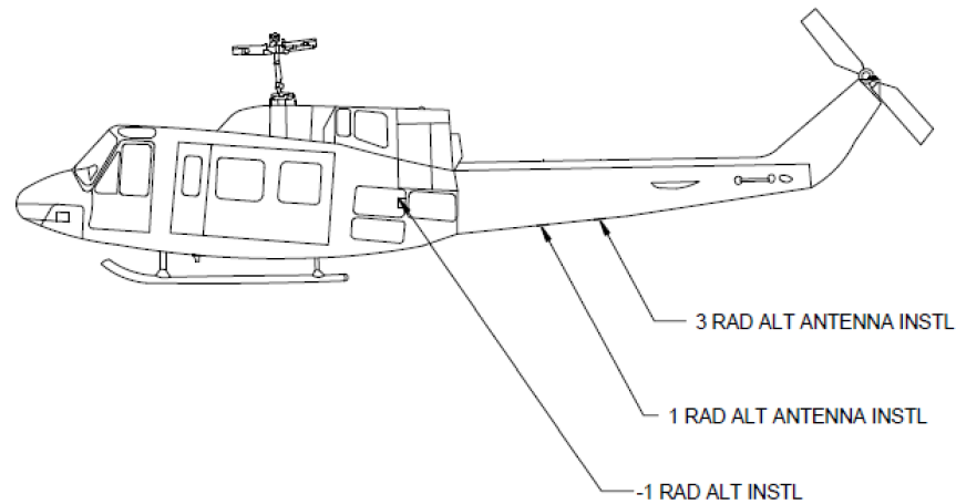
Figure 97-4 – RAD ALT System Location
