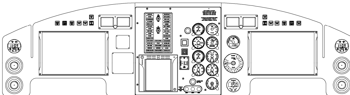
Figure 95-1 – Instrument Panel Installation (E2006-01-1-1).
