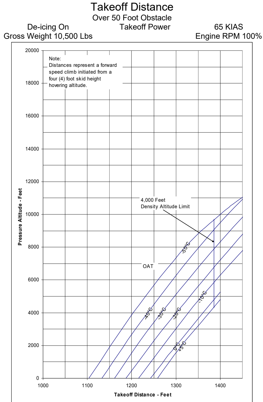
Figure 5-7 – Takeoff Distance (Sheet 10 of 12)
