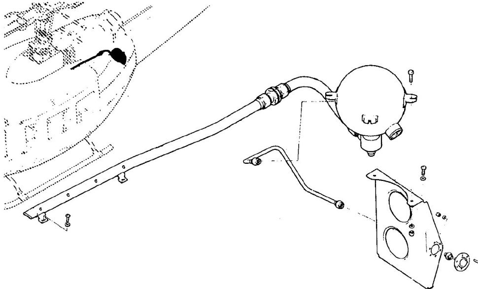
Figure 2-39 - Engine Fire Extinguisher System
