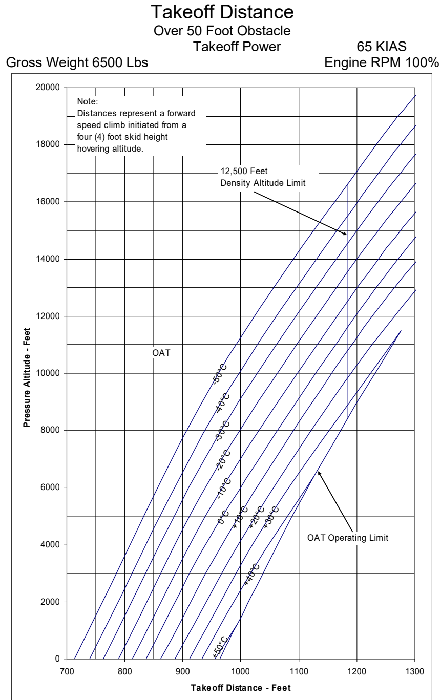
Figure 5-7 – Takeoff Distance (Sheet 1 of 12)
