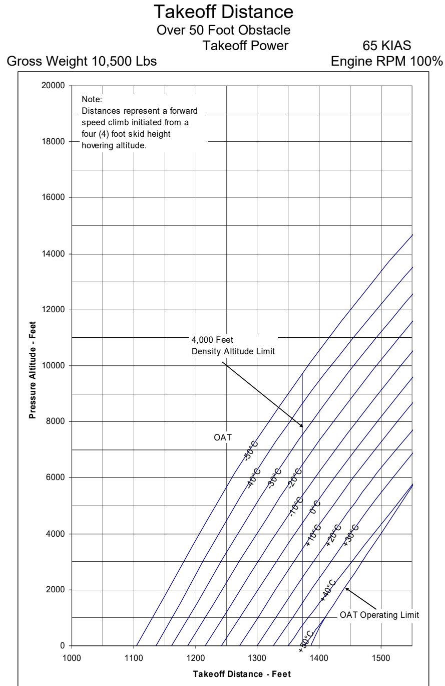
Figure 5-7 – Takeoff Distance (Sheet 9 of 12)
