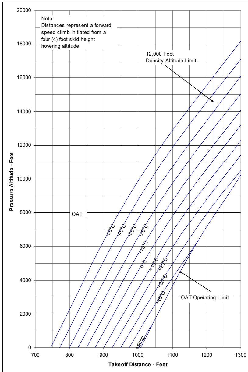
Figure 5-7 – Takeoff Distance (Sheet 5 of 12)
