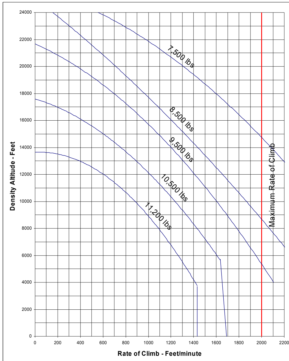
Figure 5-8 – Rate of Climb – Maximum (Sheet 1 of 2)
