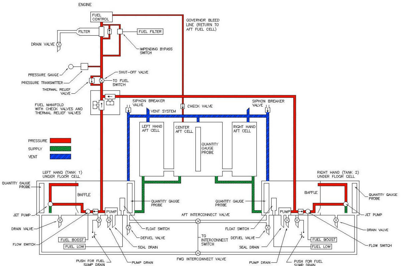
Figure 2-25 - Fuel System Pictorial Schematic
