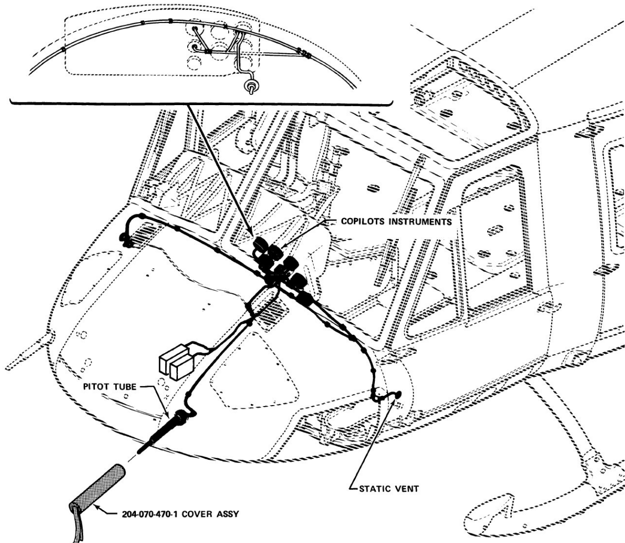
Figure 2-36 - Pitot-Static System - Optional
