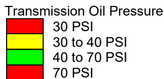
Figure 4-11 – Instrument Markings (Sheet 3 of 6)
