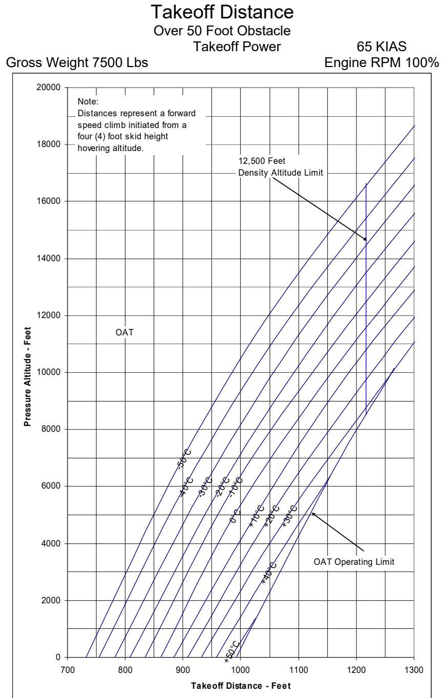
Figure 5-7 – Takeoff Distance (Sheet 3 of 12)
