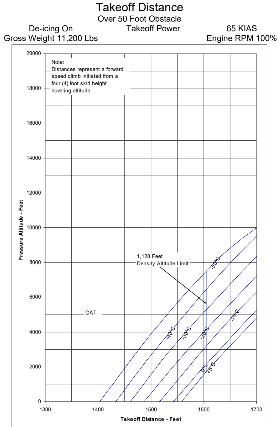
Figure 5-7 – Takeoff Distance (Sheet 12 of 12)
