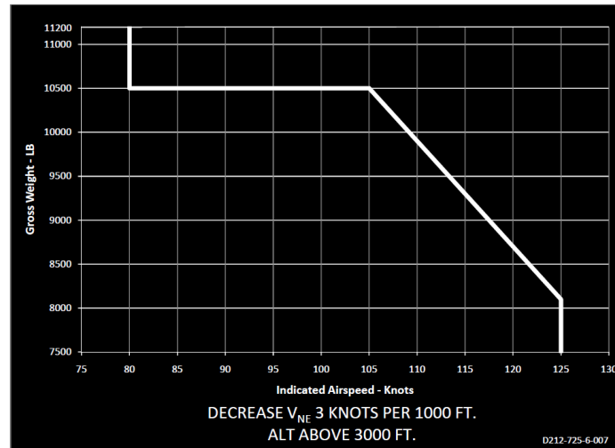
Figure 4-6A – VNE Placard
