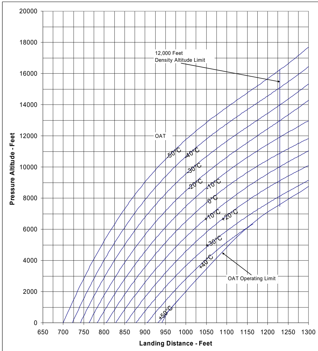
Figure 5-9 – Landing Distance (Sheet 3 of 6)
