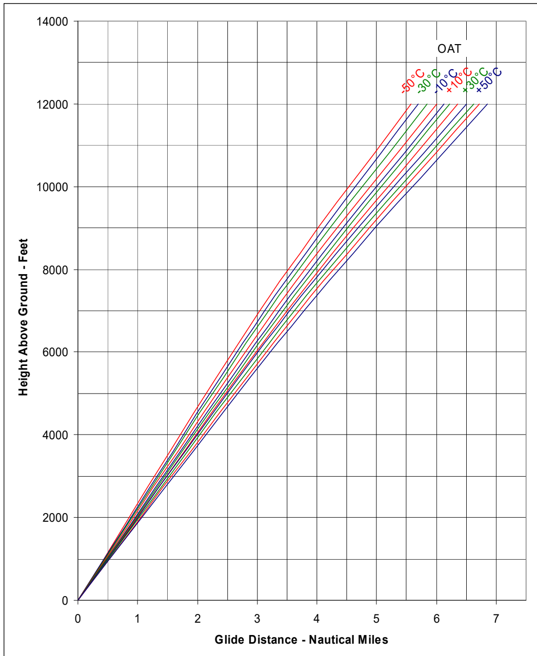
Figure 5-12 – Glide Distance
