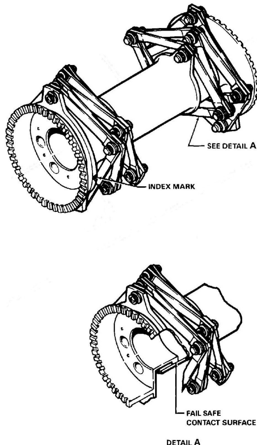
Figure 2-18 - Main Driveshaft
