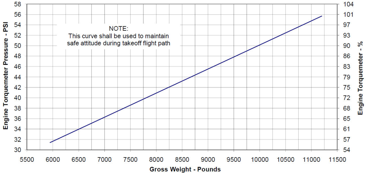
Figure 4-7 – Power Limits for Takeoff
