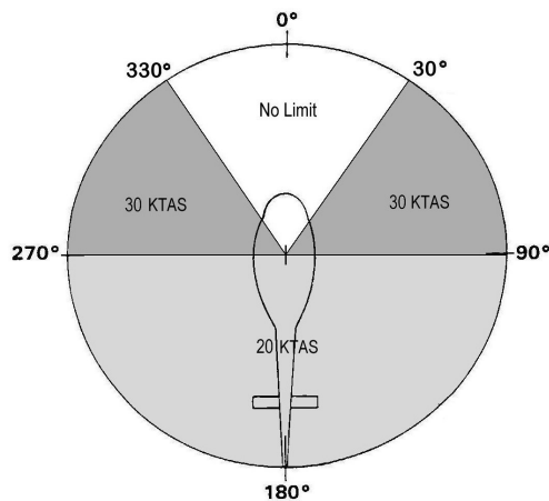
Figure 5-4 – Operation vs Allowable Wind Above 10,500 Lbs
