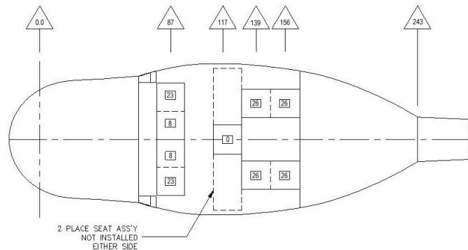
Figure 4-3 – Nine-place passenger loading configuration 3
