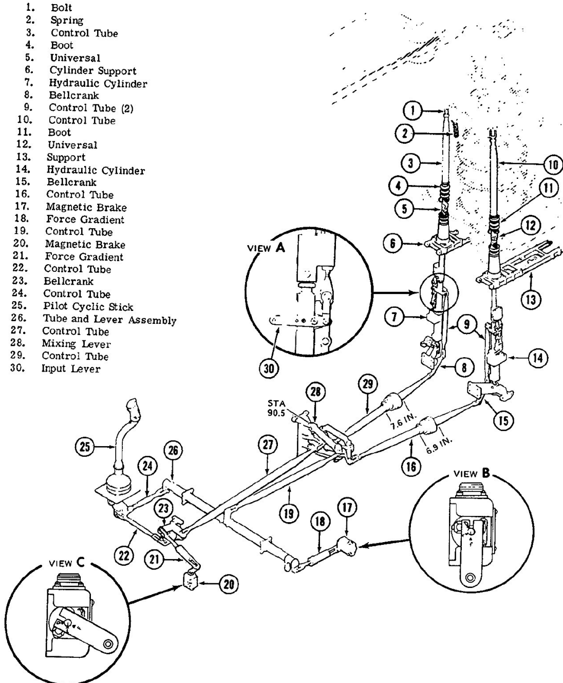
Figure 2-29 - Cyclic Control System
