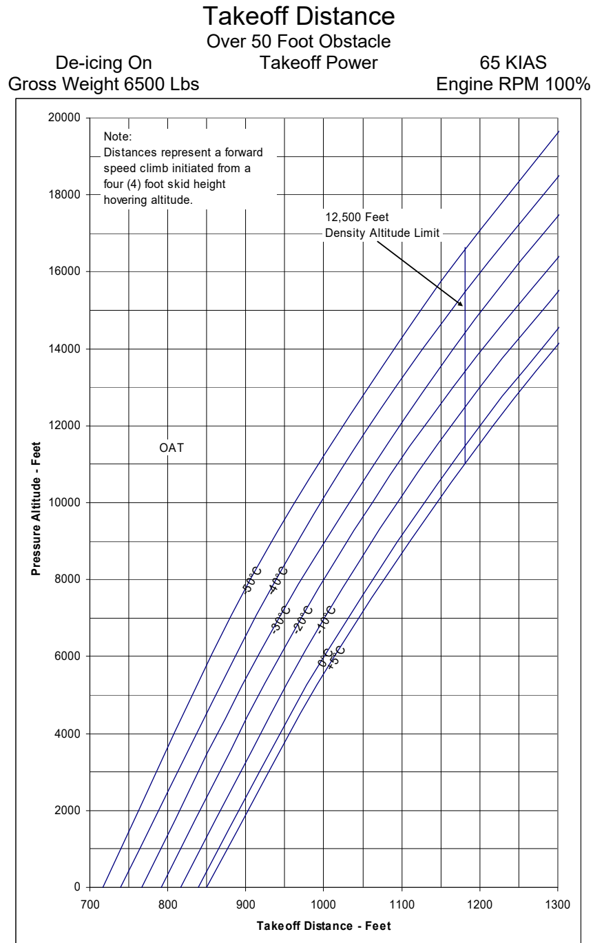
Figure 5-7 – Takeoff Distance (Sheet 2 of 12)
