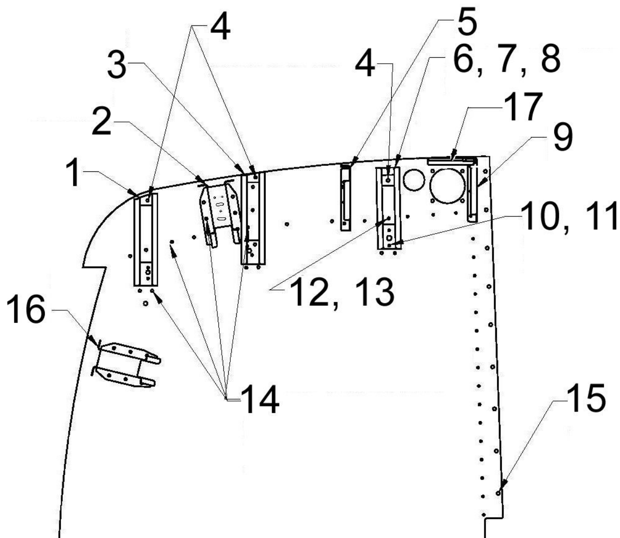
Figure 53-16 – Bulkhead Installation
