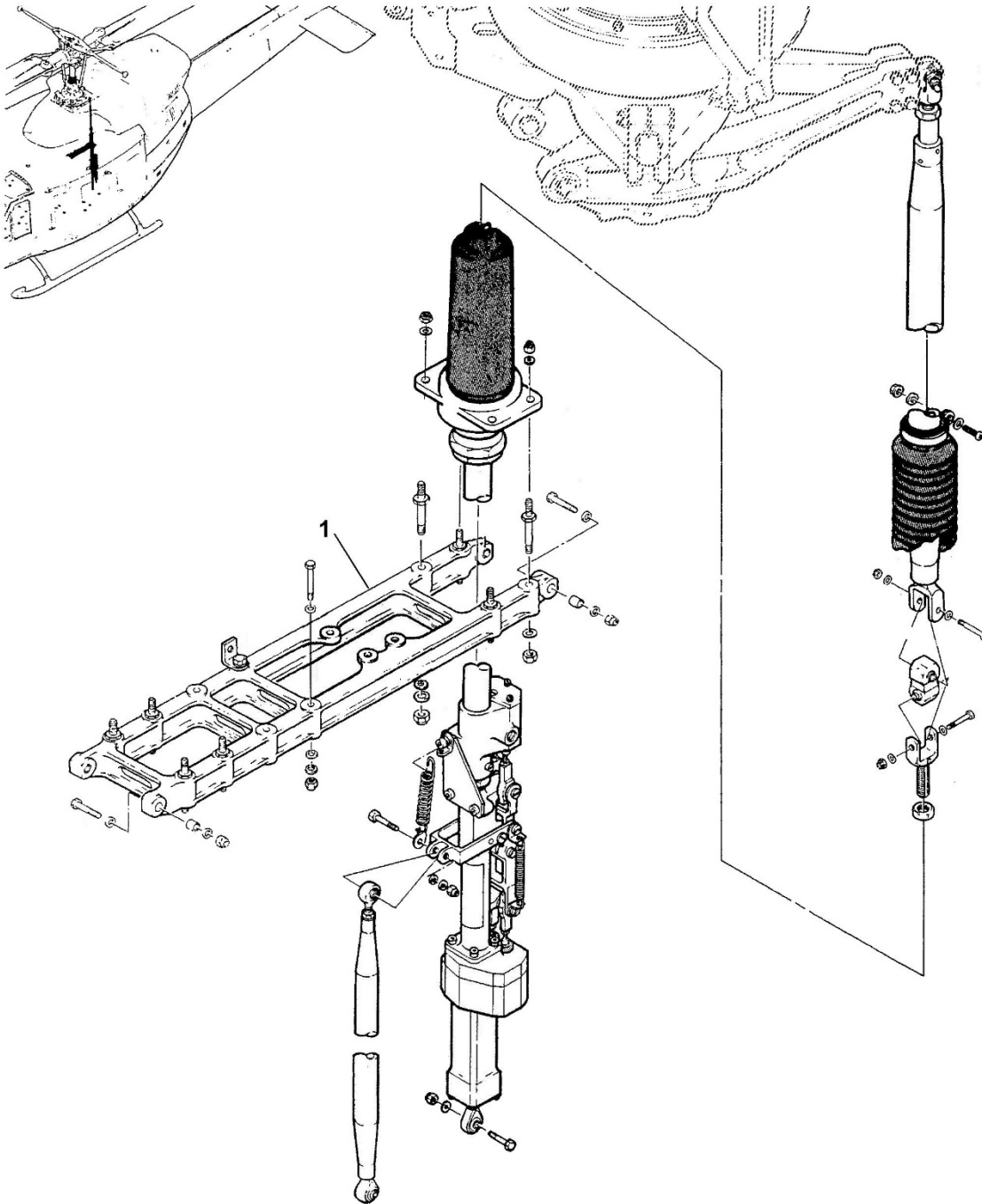
Figure 67-2 – Collective Installation – Servo
