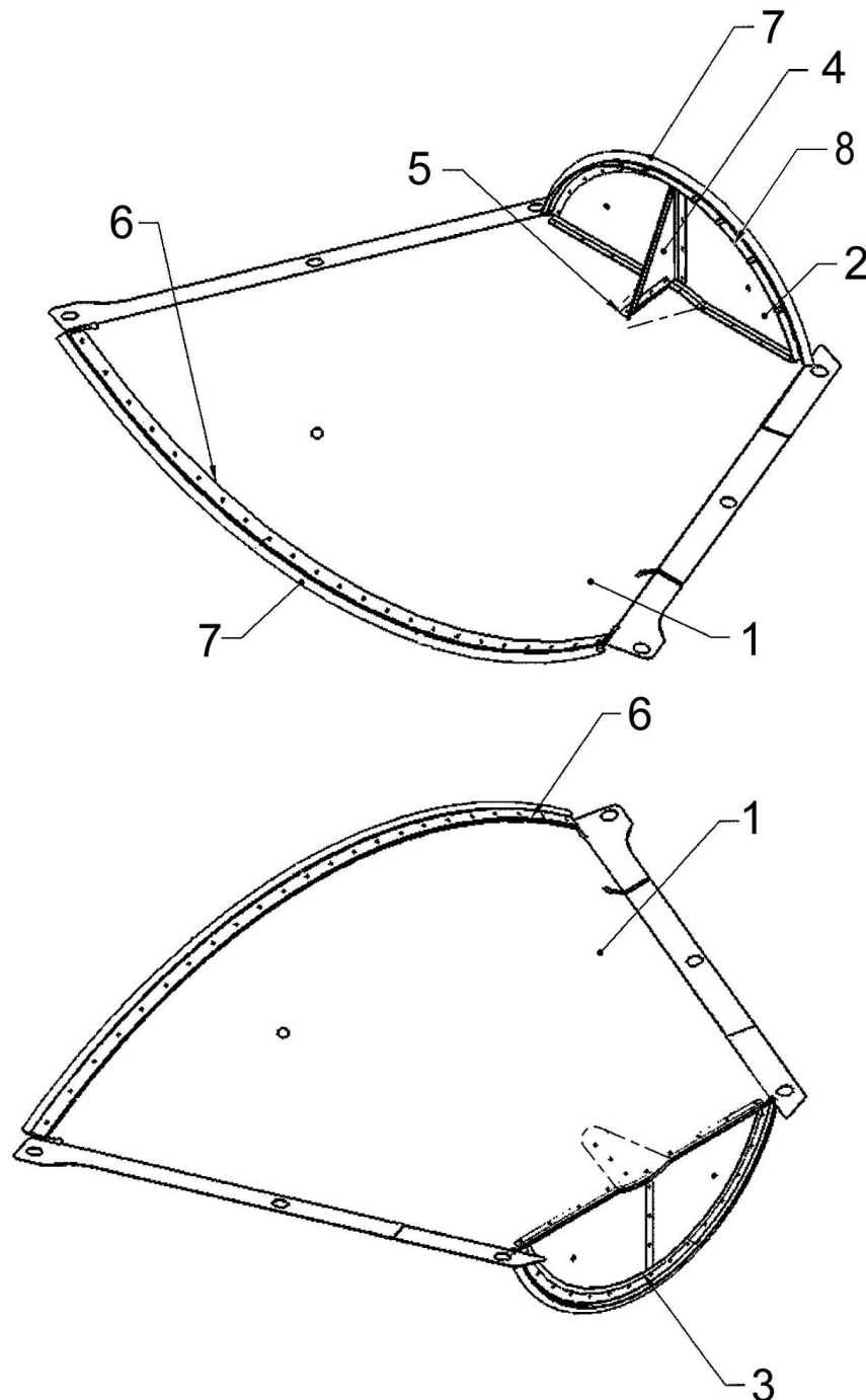
Figure 53-29 – D212-725-1-939 Tail Pipe Shield
