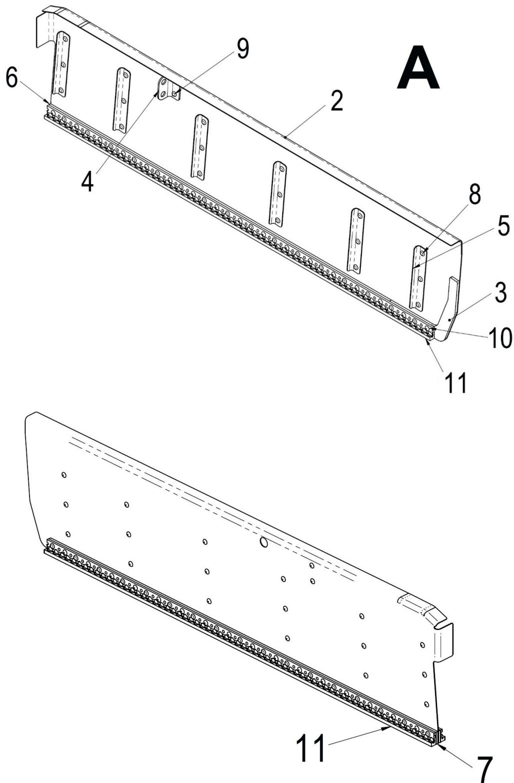
Figure 53-31 – Roof Installation, Cabin (Sheet 2 of 2)
