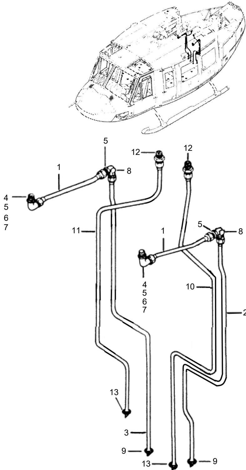
Figure 53-12 – Drain Installation
