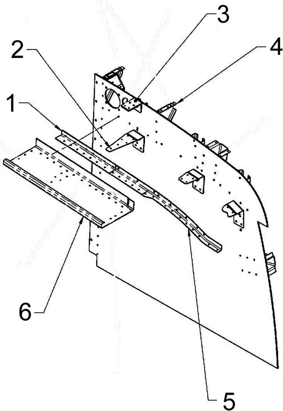
Figure 53-17 – Bulkhead Installation
