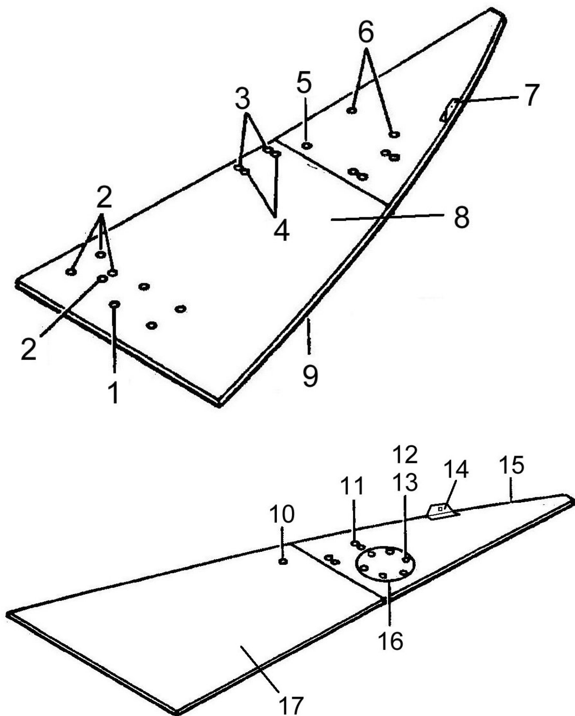
Figure 53-15 – Engine Side Service Decks
