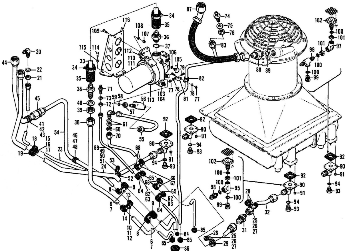
Figure 79-3 – Oil System Installation
