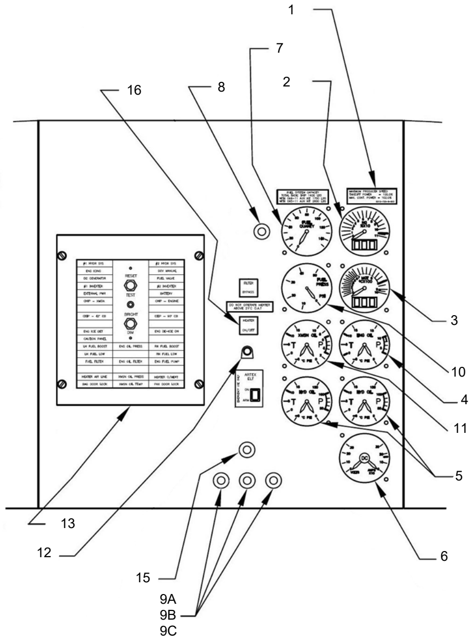
Figure 95-5 - Instrument Panel (Center)
