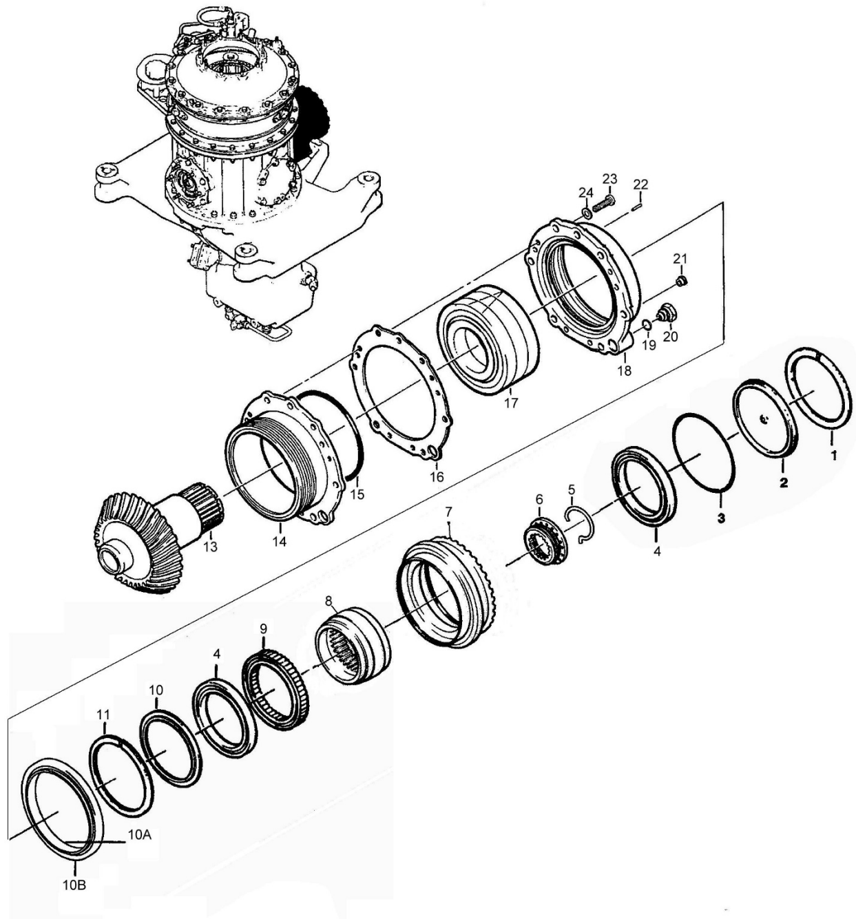
Figure 63-4 - 205-040-263-101 Quill Assembly
