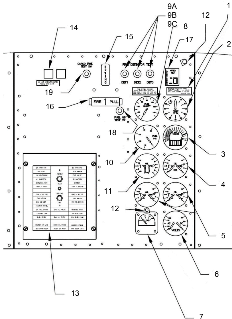
Figure 95-2 - Instrument Panel (Center)
