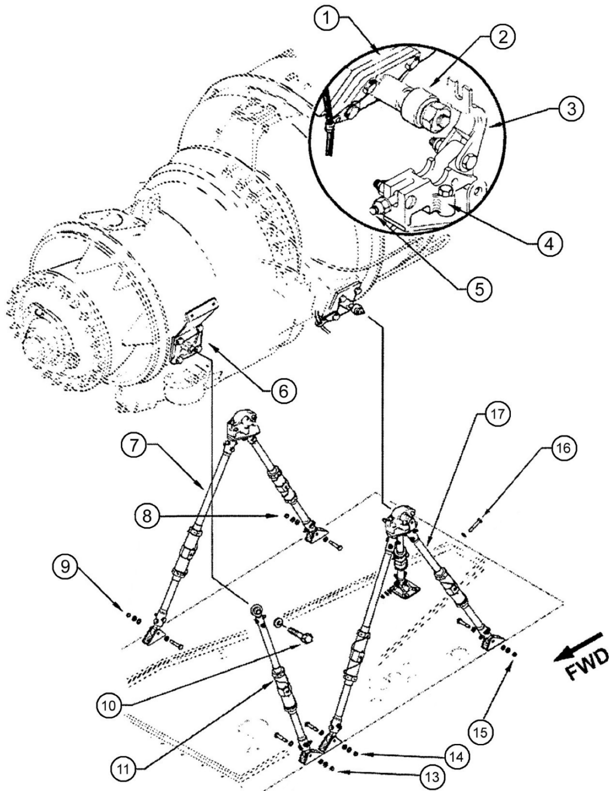
Figure 71-16 - Engine Mount Assembly
