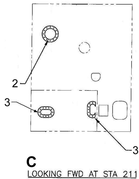
Figure 53-14 – Bulkhead, Tension Rod, Support Installation and Bulkhead Detail (Sheet 2 of 2)
