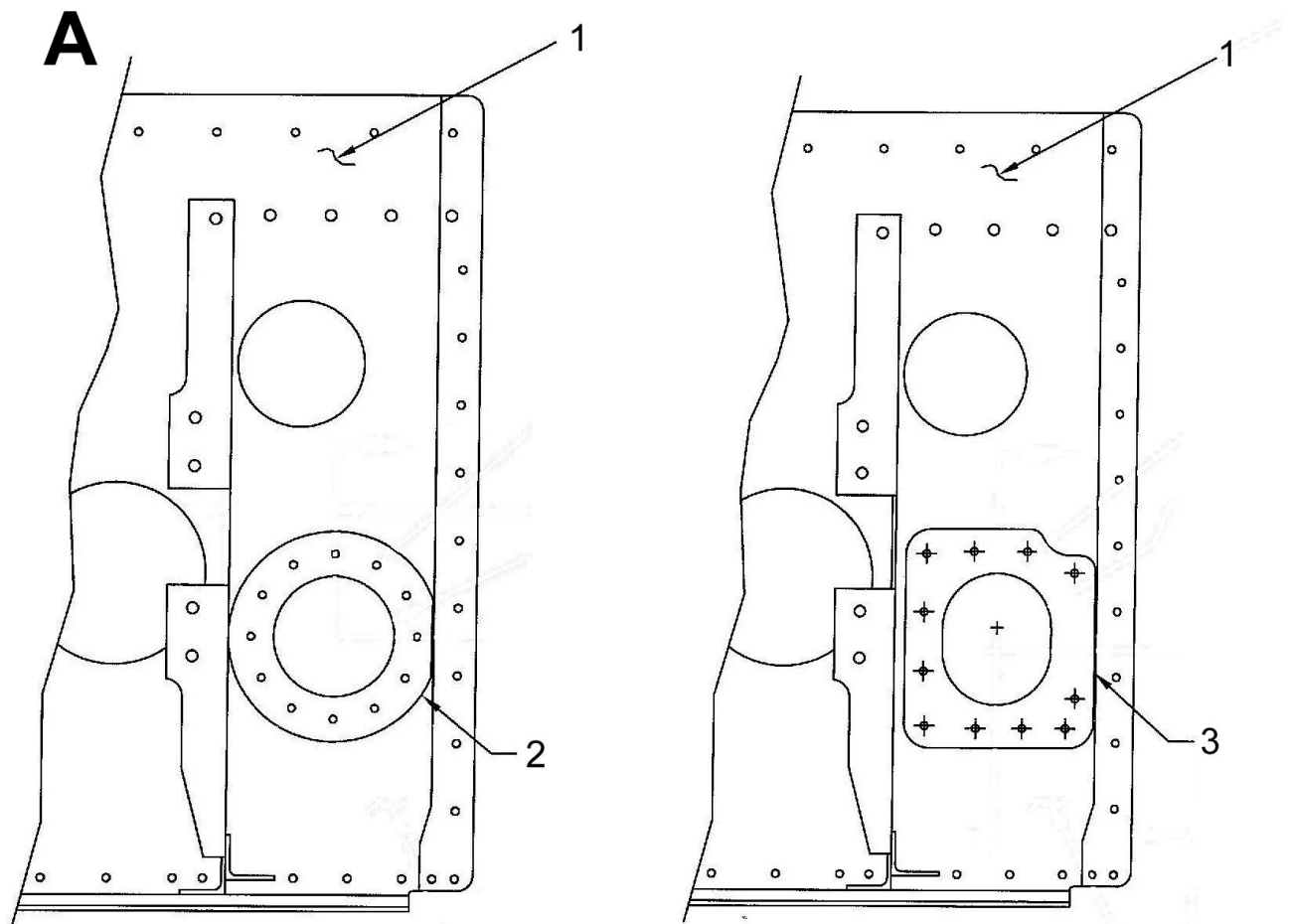
Figure 53-22 – Bulkhead Detail (Sheet 2 of 2)
