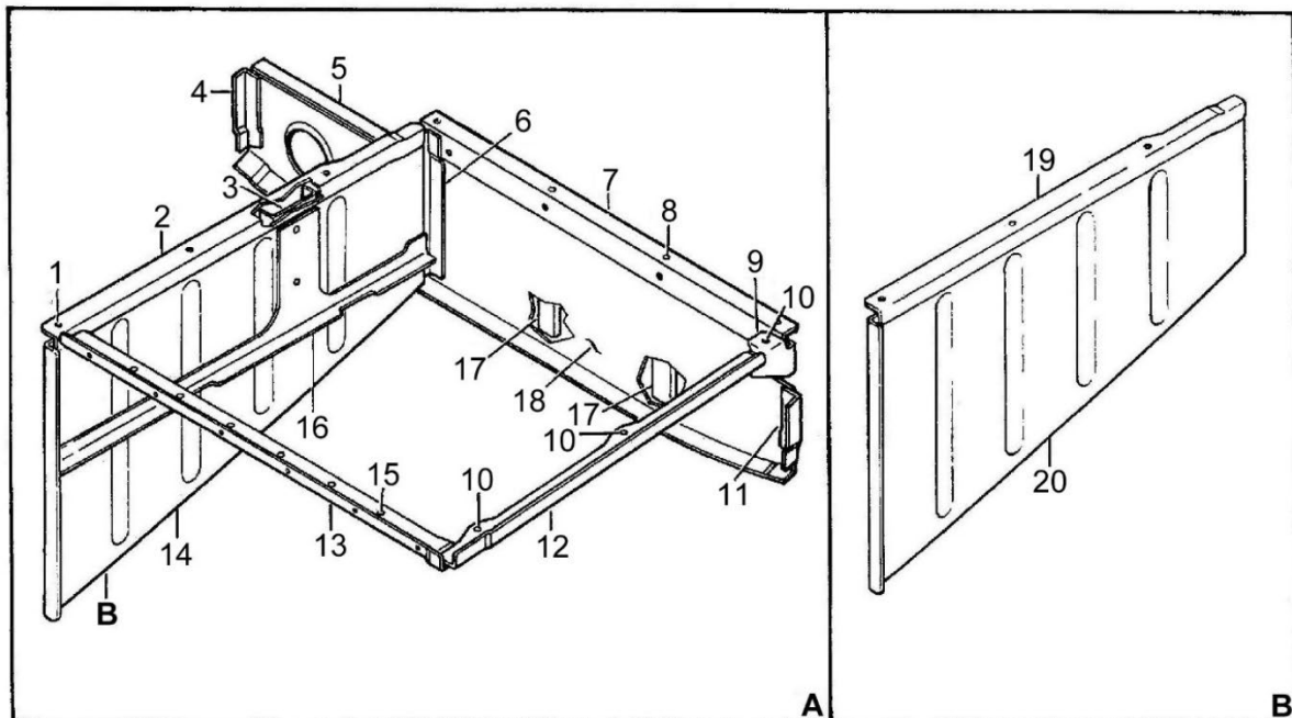
Figure 53-19 – Oil Cooler Support
