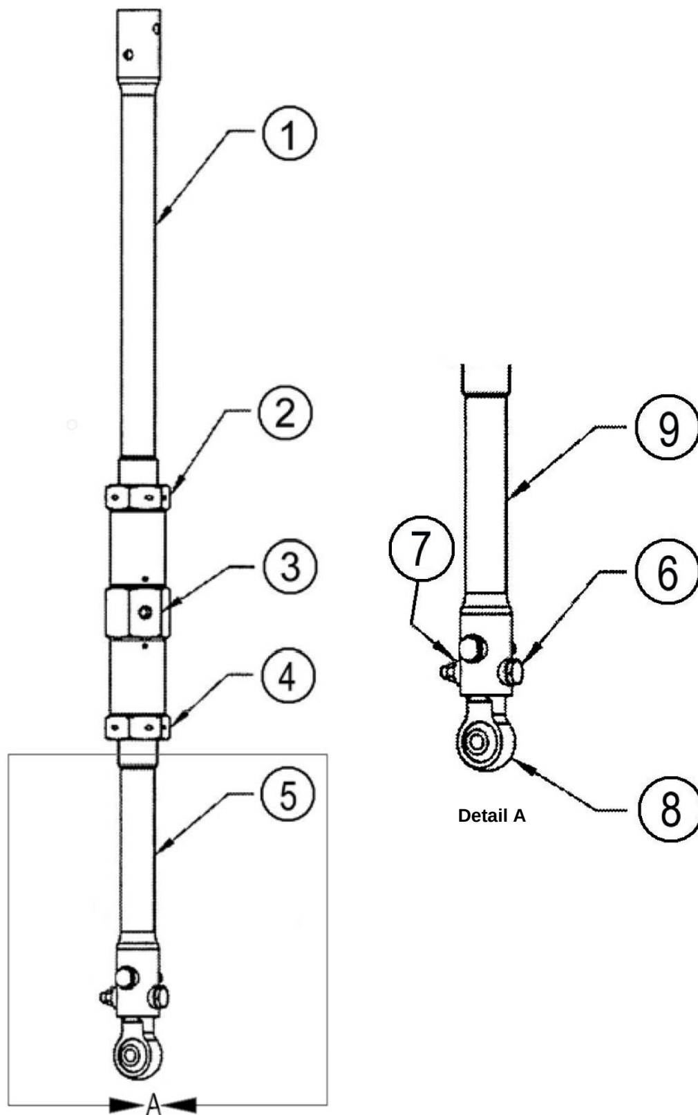
Figure 71-17 - Engine Mount Detail (Bipod and Tripod) (Sheet 1 of 2)
