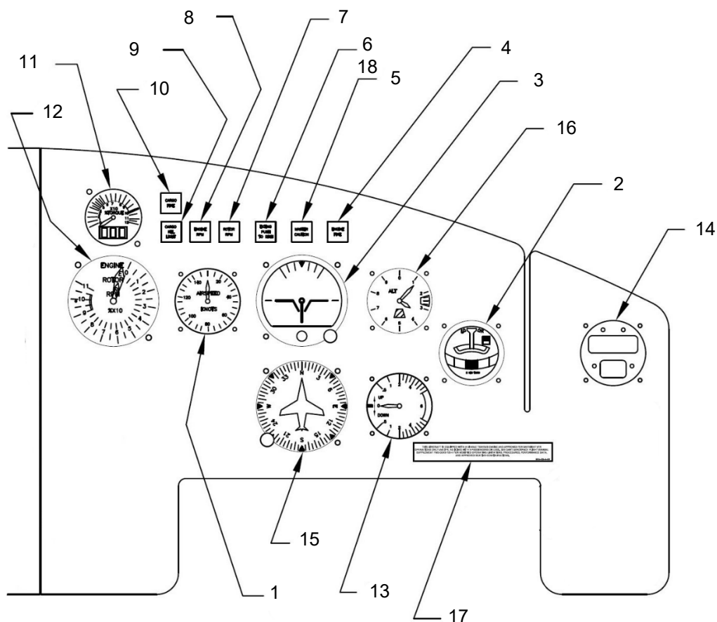
Figure 95-6 — Instrument Panel (RH)
