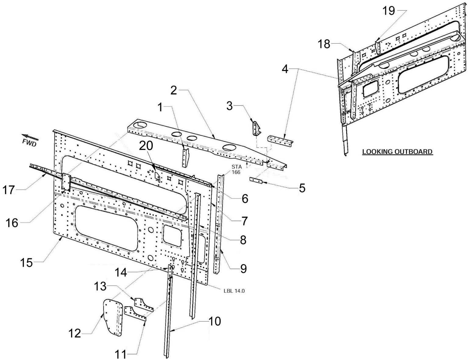
Figure 53-6 – Pylon Web
