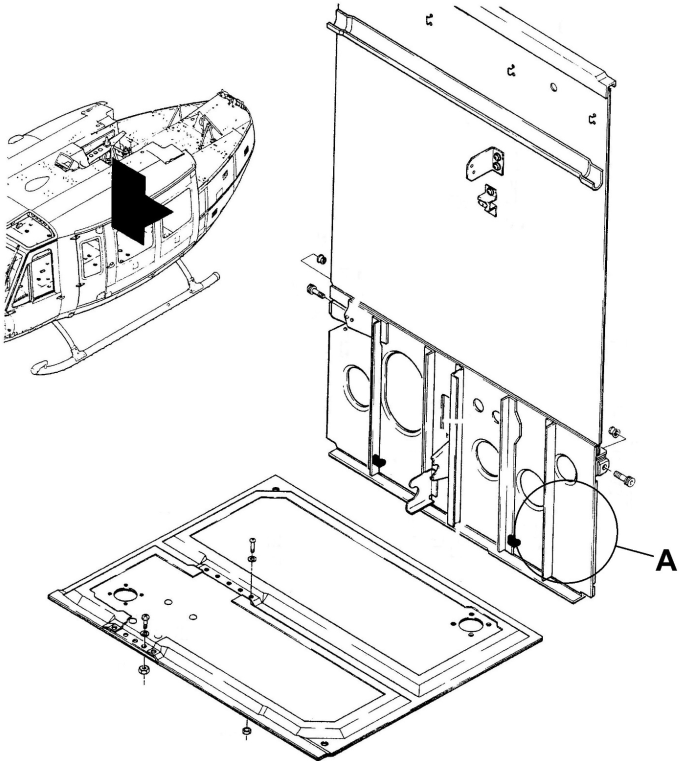
Figure 53-21 – Bulkhead Detail (Sheet 1 of 2)
