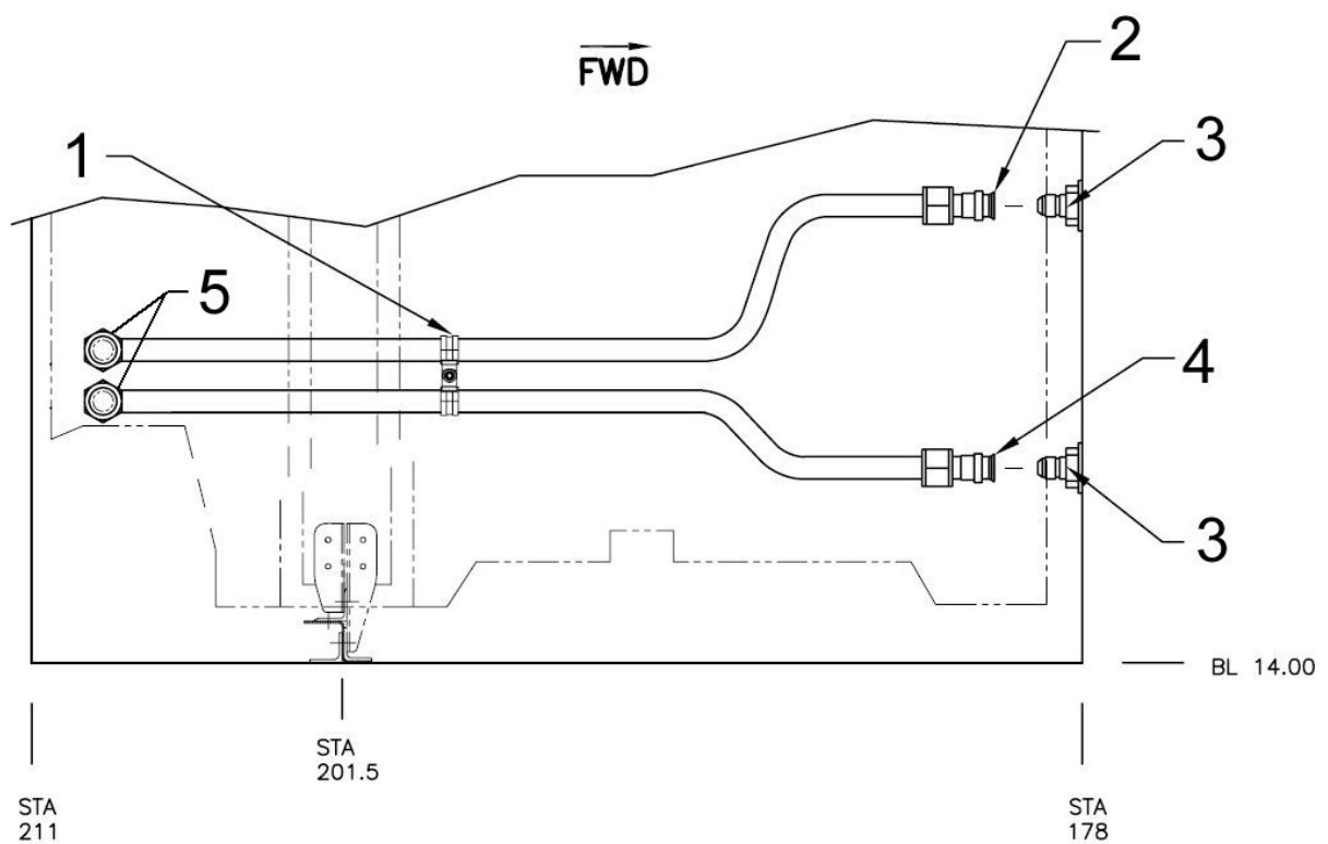
Figure 53-27 – Vent Tube Installation
