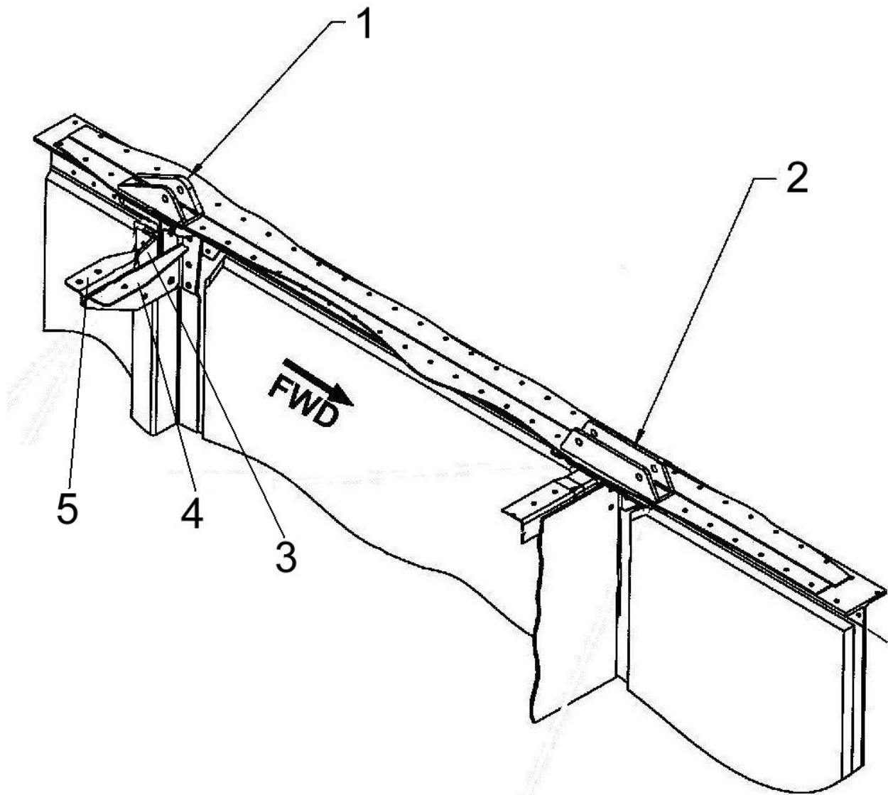
Figure 53-20 – Engine Mount Detail
