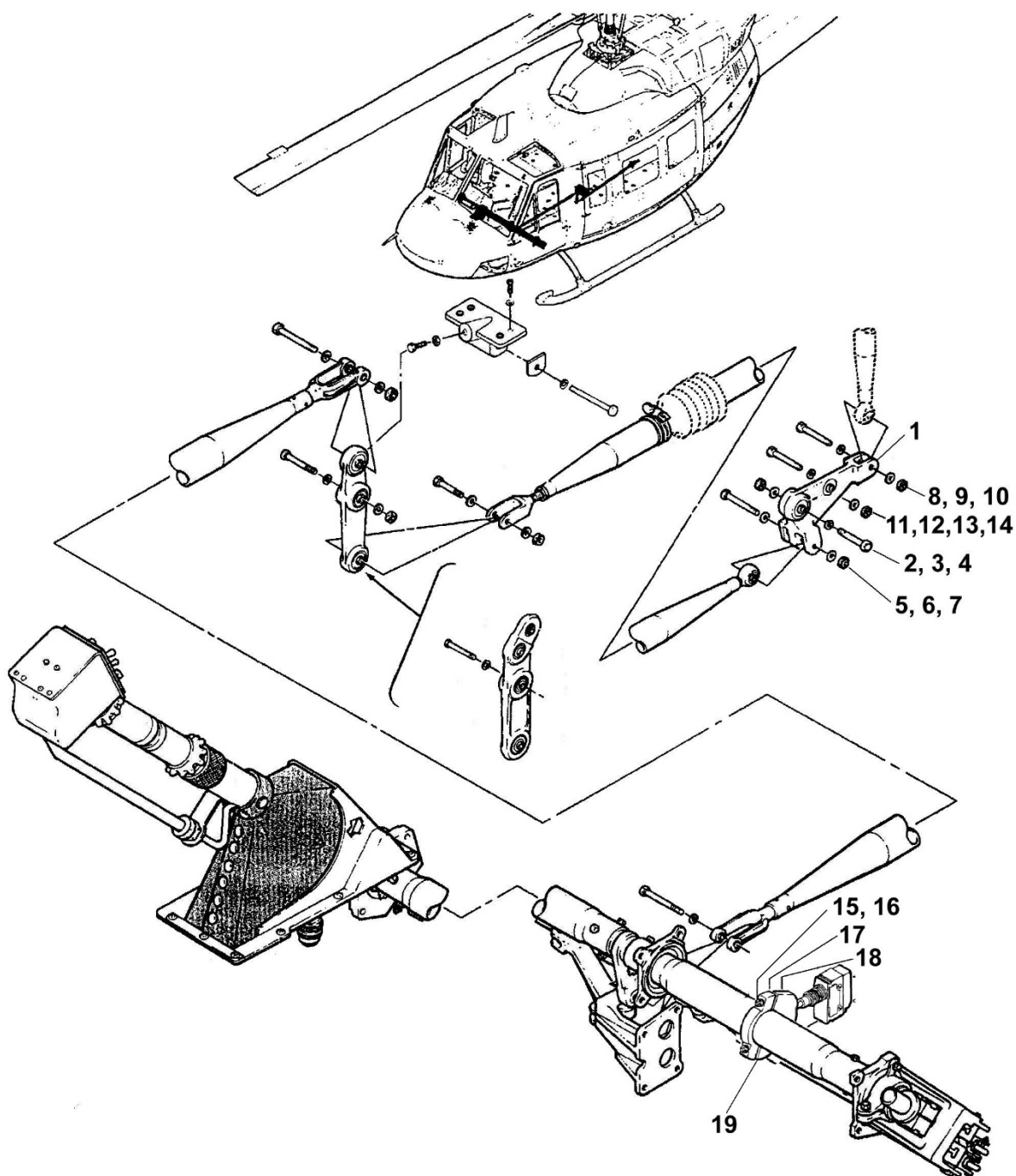
Figure 67-1 – Collective Installation – Forward Cabin
