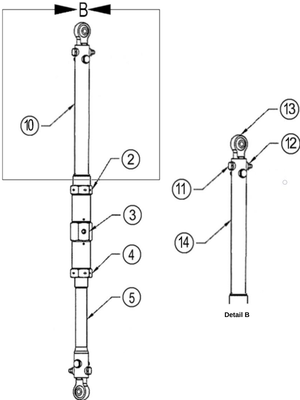
Figure 71-18 – Engine Mount Detail (Monopod) (Sheet 2 of 2)
