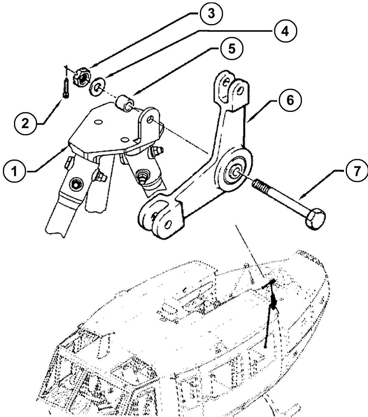
Figure 71-19 - Throttle Lever Installation
