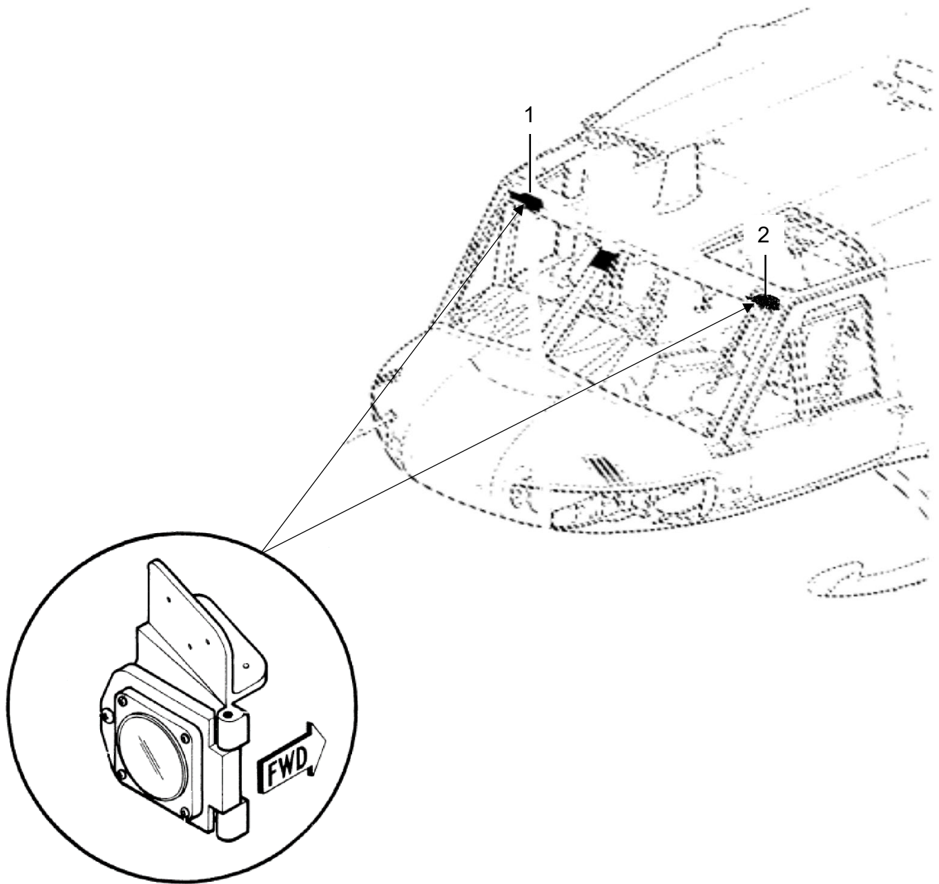
Figure 95-7 - Standby Compass Bracket Assembly
