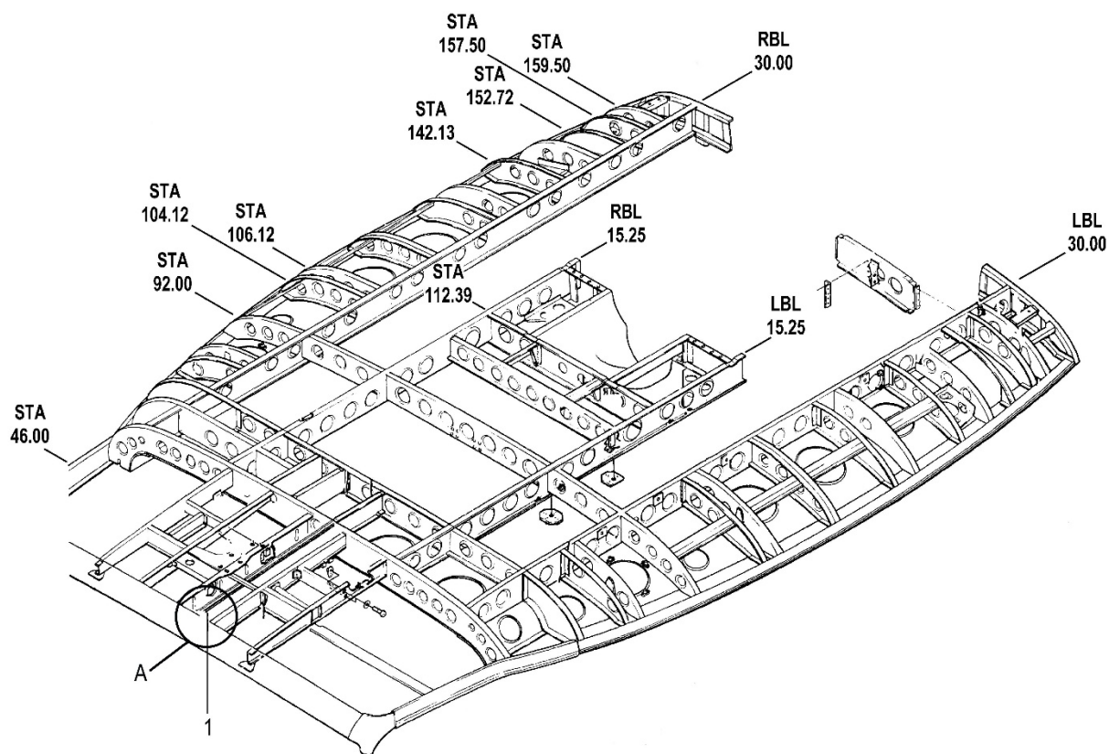
Figure 53-30 – Roof Installation (Sheet 1 of 2)
