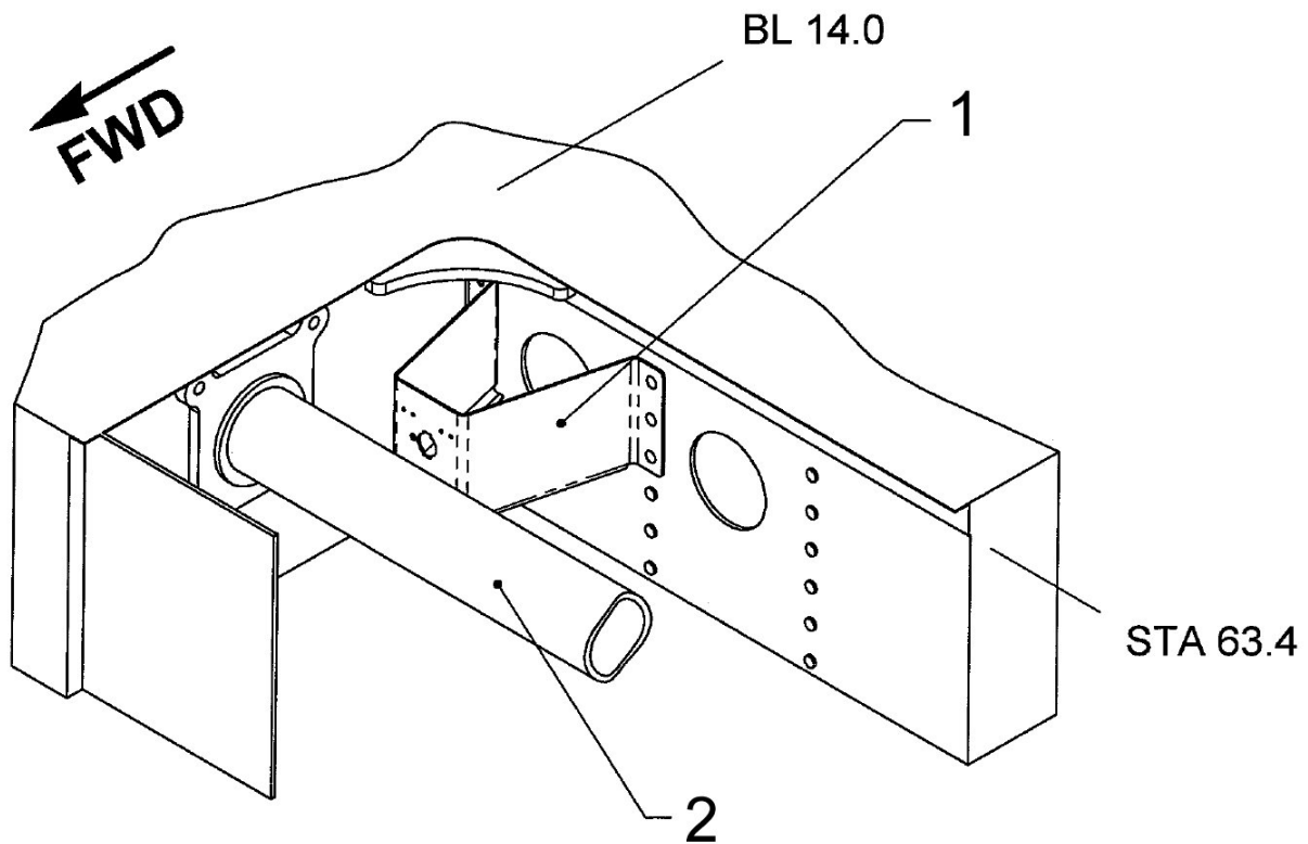
Figure 53-25 – D212-725-1-061 Bracket Installation
