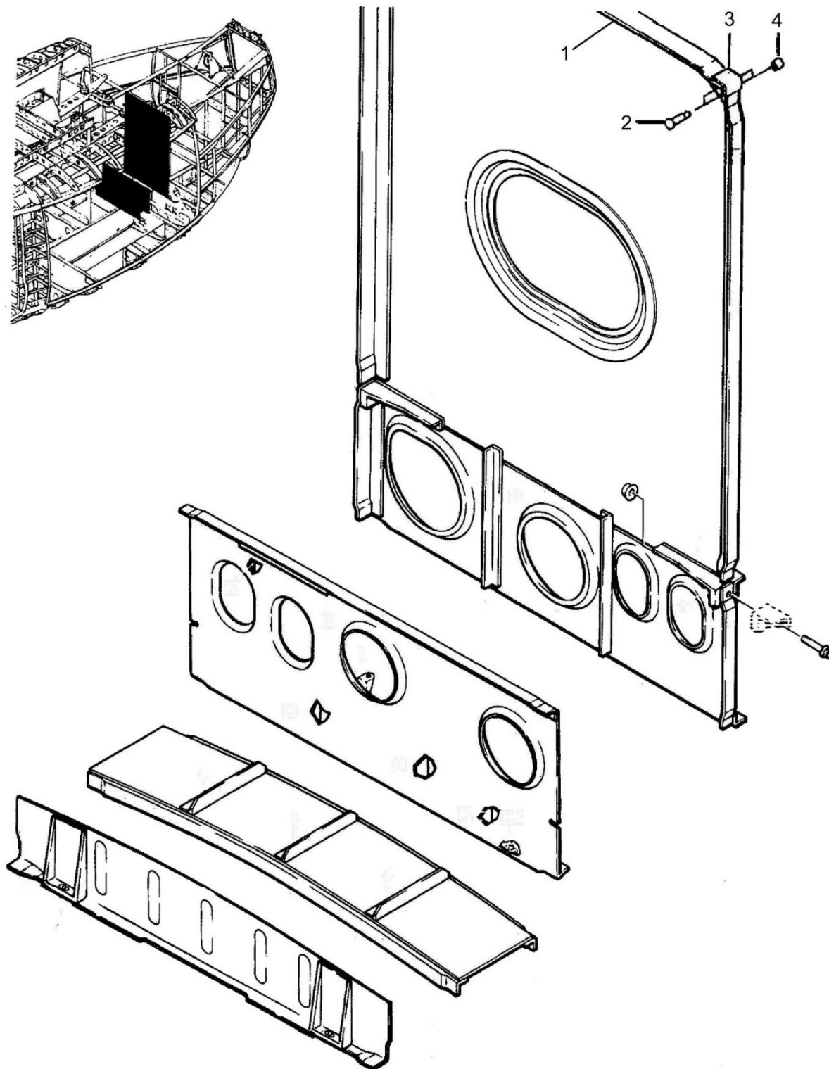
Figure 53-18 – Bulkhead and Cover Installation
