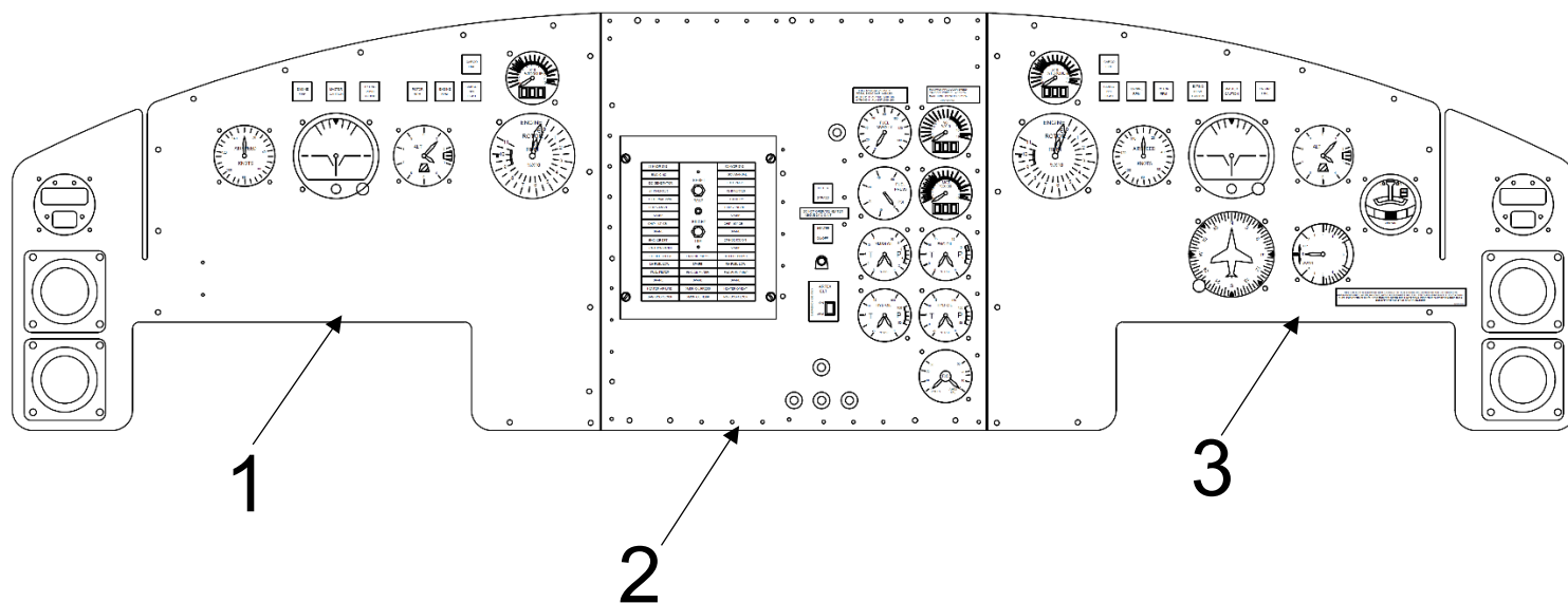
Figure 53-35 - Instrument Panel Assembly
