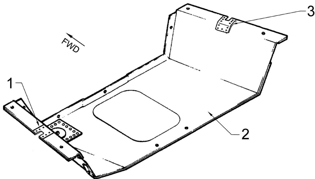
Figure 53-28 – D212-725-1-201 Doubler Installation
