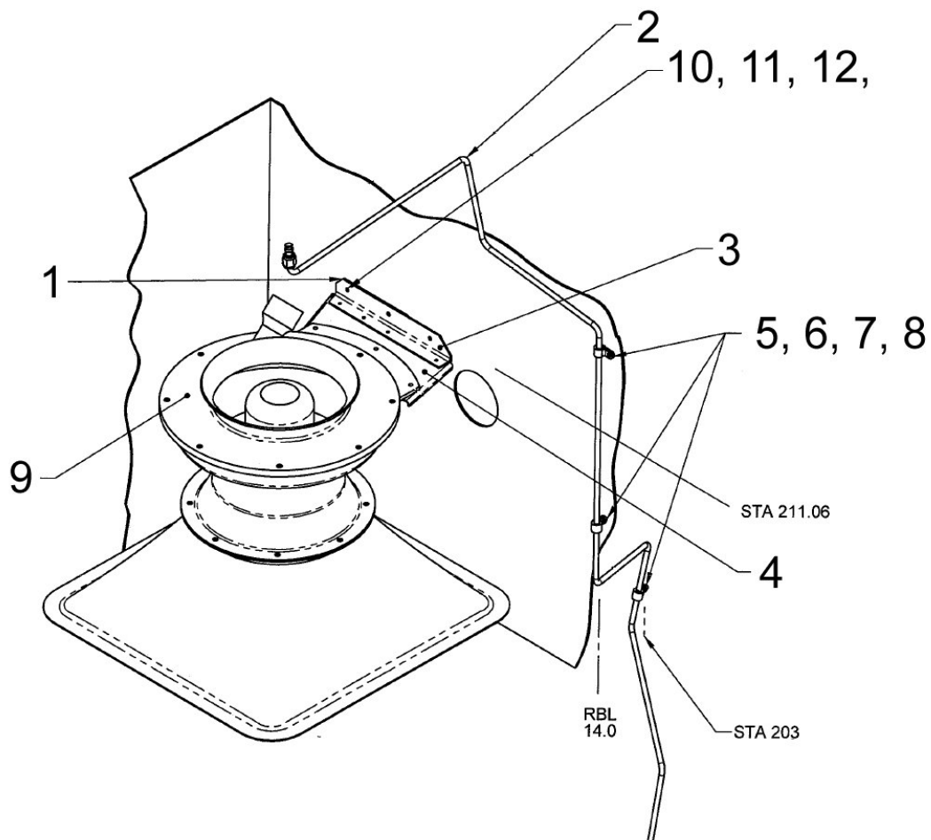
Figure 53-24 – Oil Cooler Installation
