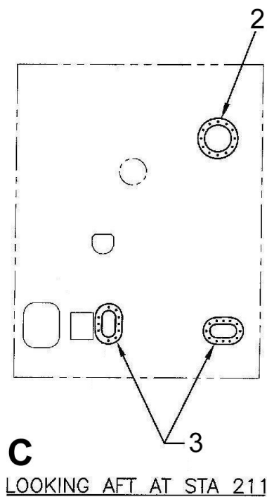
Figure 53-14 – Bulkhead, Tension Rod, Support Installation and Bulkhead Detail (Sheet 2 of 2)
