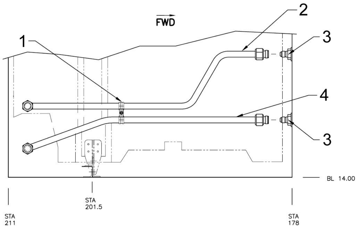
Figure 53-26 – Vent Tube Installation
