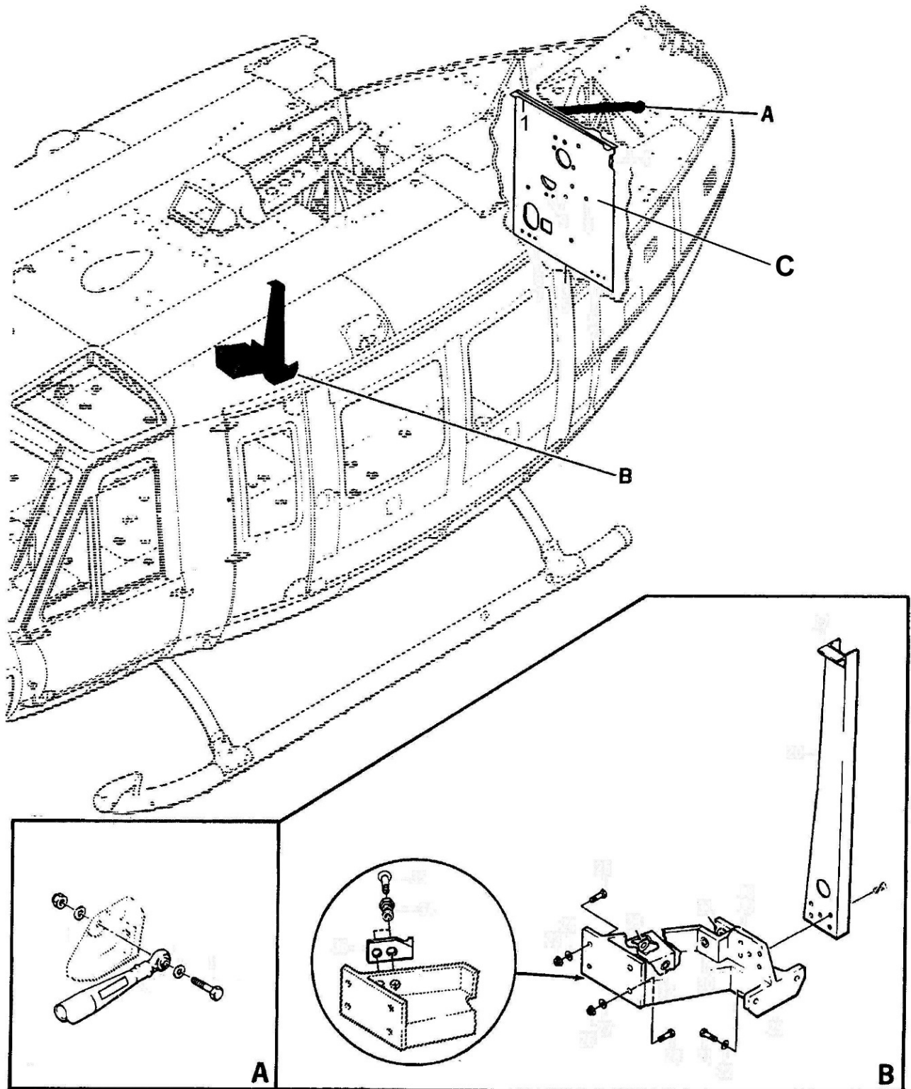
Figure 53-13 – Bulkhead, Tension Rod, Support Installation and Bulkhead Detail (Sheet 1 of 2)
