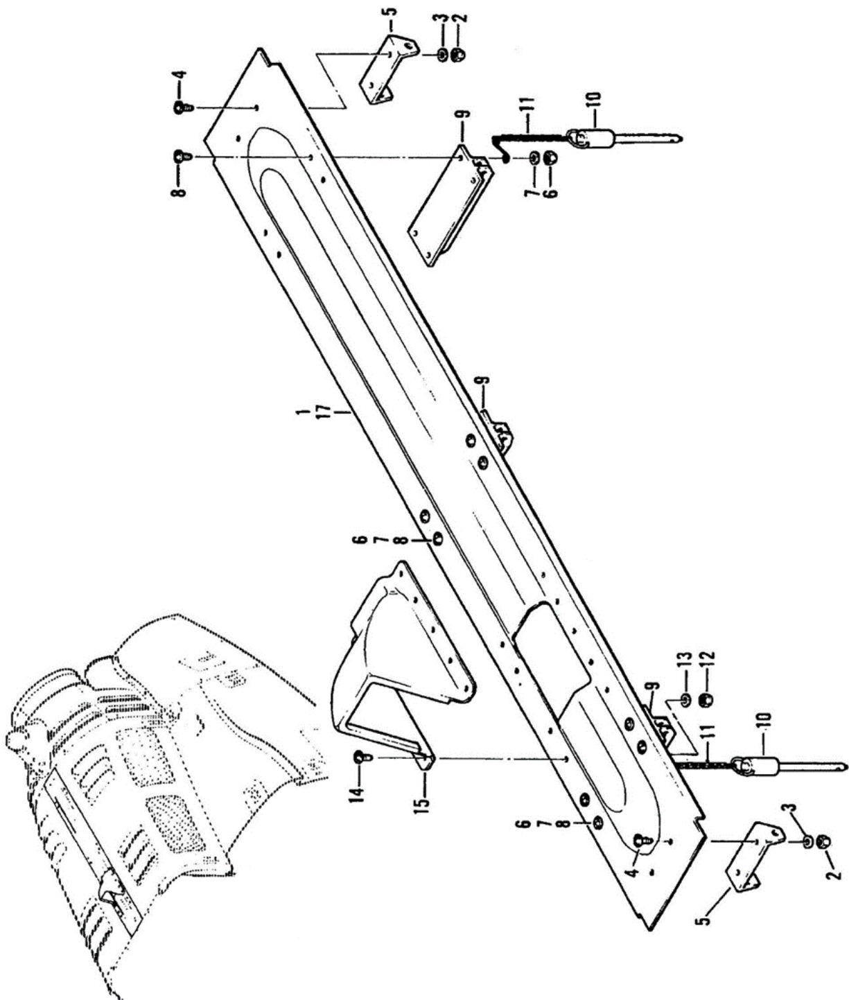
Figure 71-2 – Cowl Installation
