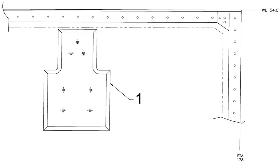
Figure 53-23 – Idle Stop Mount
