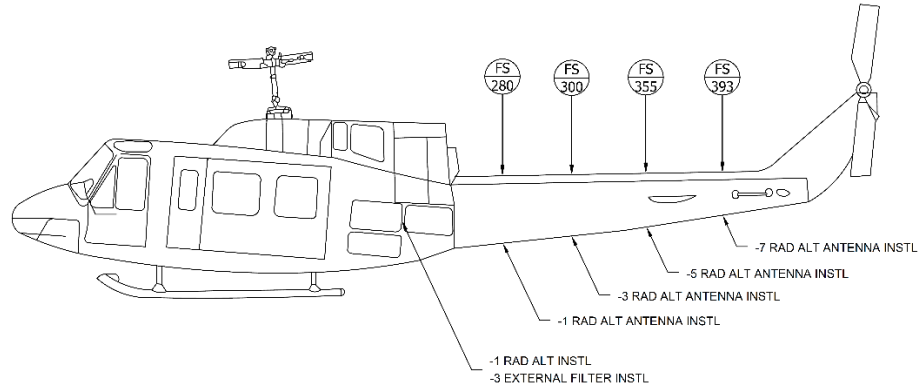
Figure 97-4 – RAD ALT System Location
