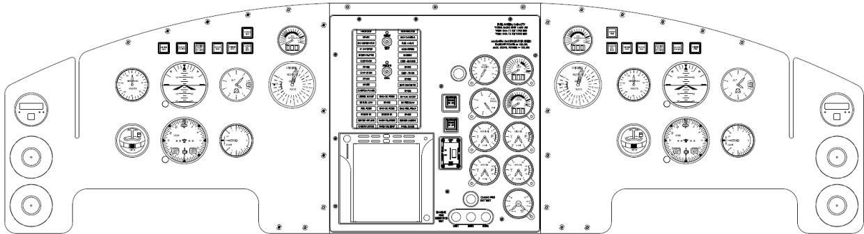
Figure 95-3 - Instrument Panel Installation (E2006-01-1-5).
